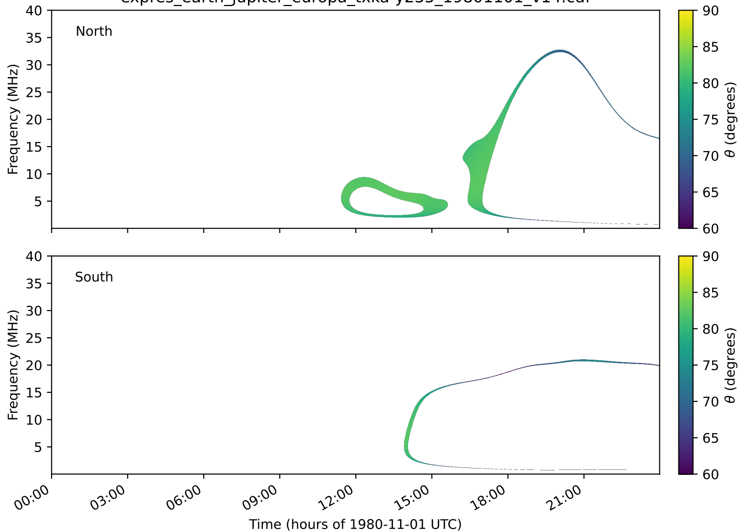
expres_earth_jupiter_europa_txka-y235_19801101_v14.cdf
