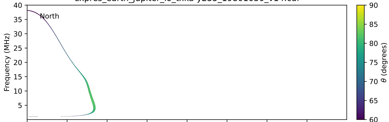
expres_earth_jupiter_io_txka-y235_19801030_v14.cdf
