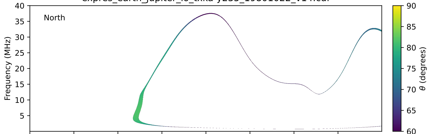
expres_earth_jupiter_io_txka-y235_19801022_v14.cdf
