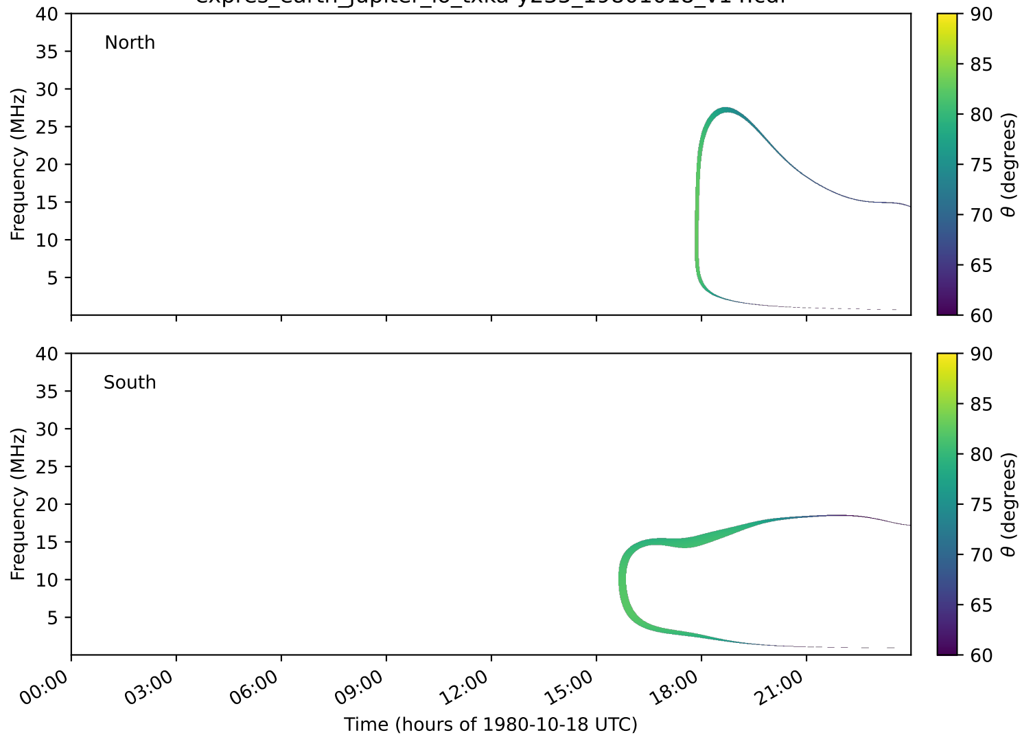
expres_earth_jupiter_io_txka-y235_19801018_v14.cdf
