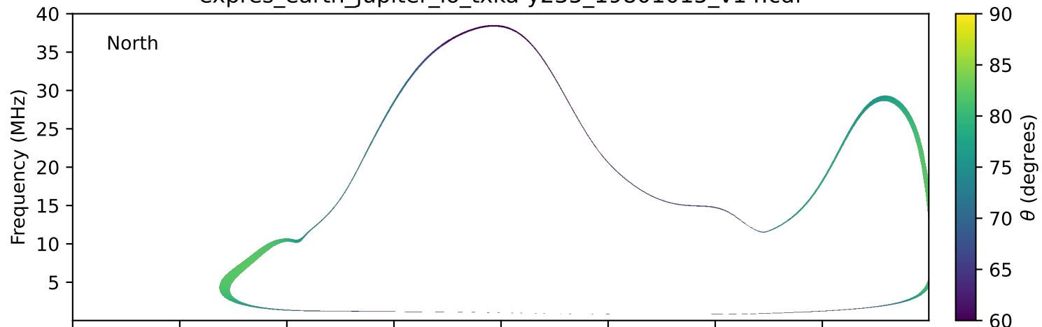
expres_earth_jupiter_io_txka-y235_19801015_v14.cdf
