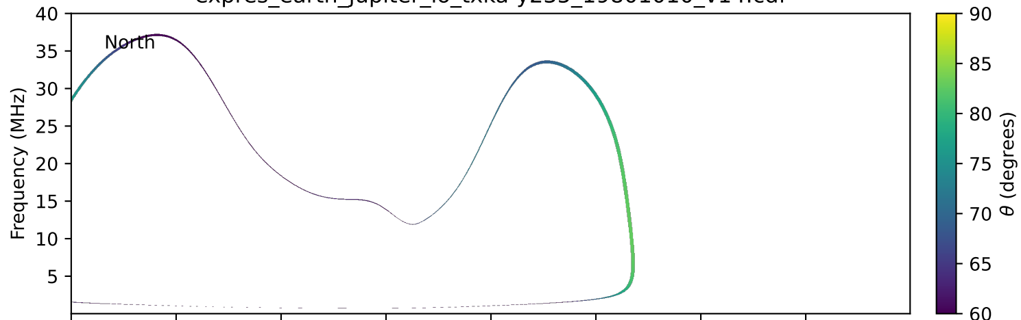
expres_earth_jupiter_io_txka-y235_19801010_v14.cdf
