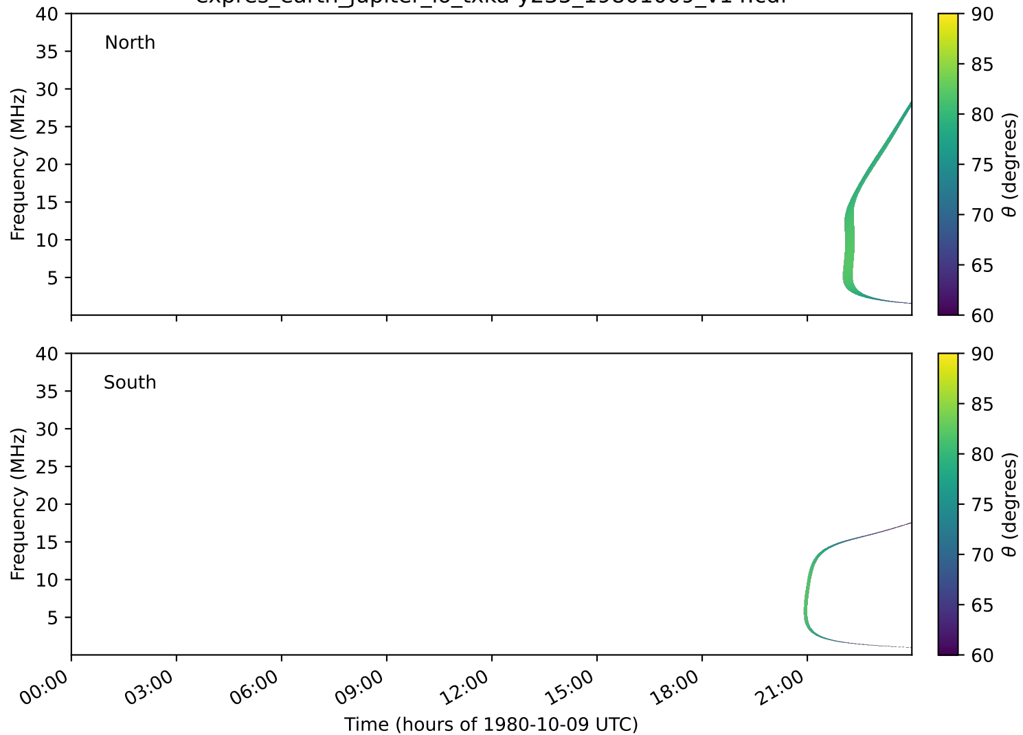
expres_earth_jupiter_io_txka-y235_19801009_v14.cdf
