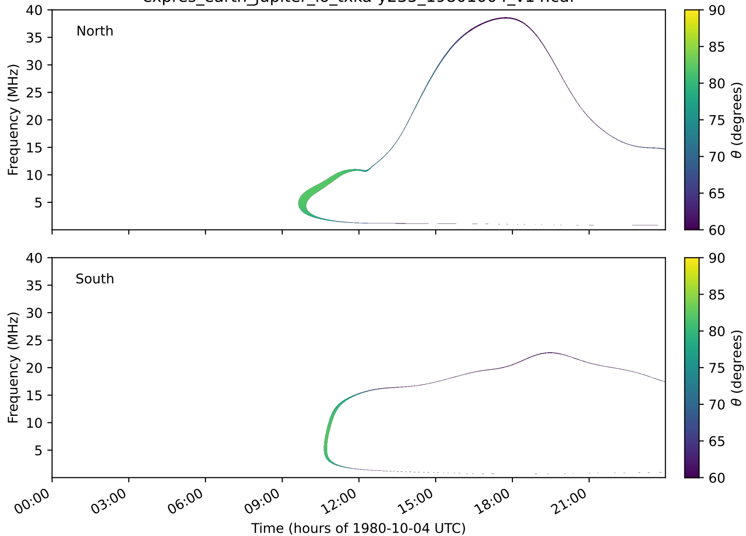
expres_earth_jupiter_io_txka-y235_19801004_v14.cdf
