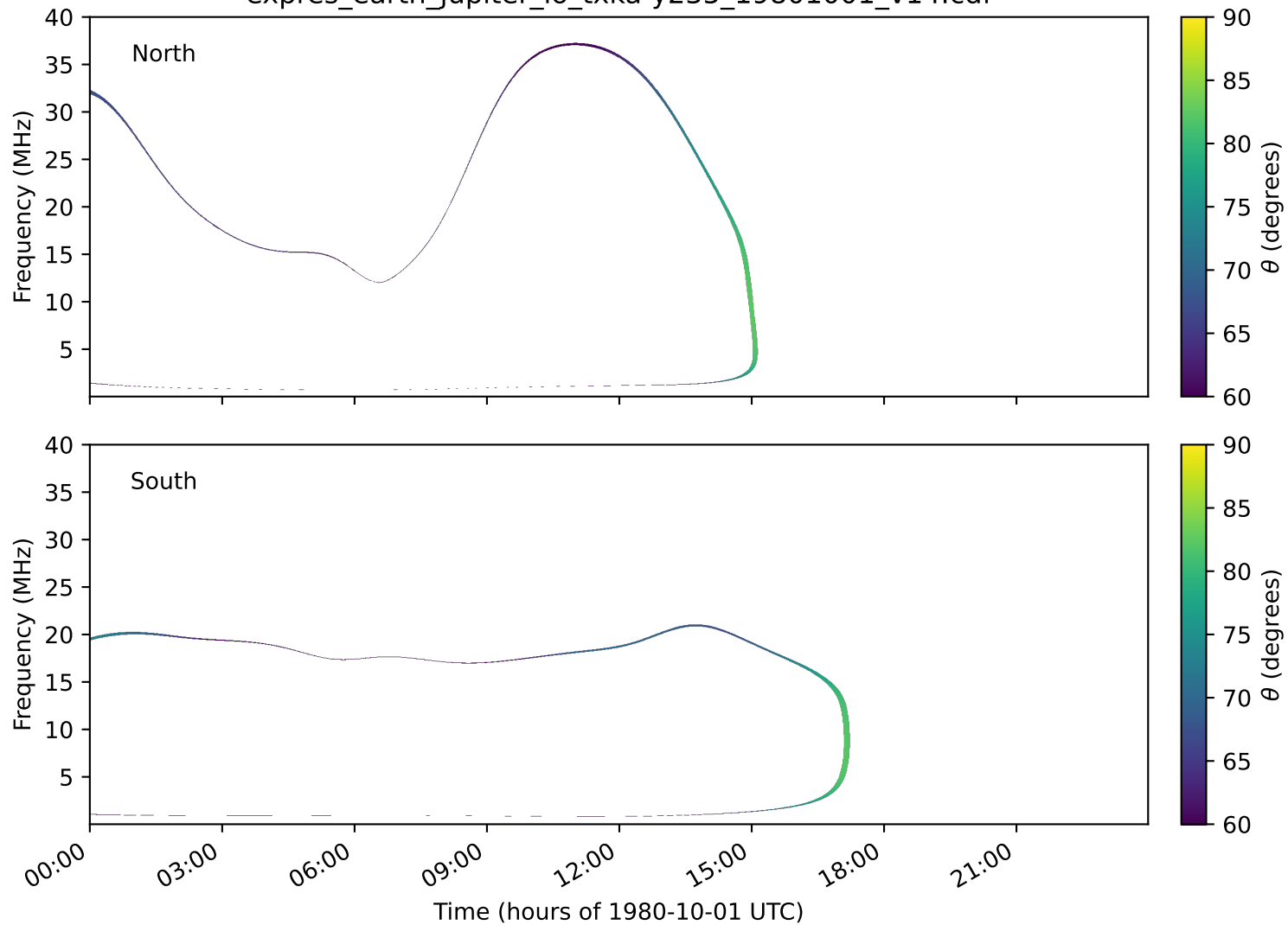
expres_earth_jupiter_io_txka-y235_19801001_v14.cdf
