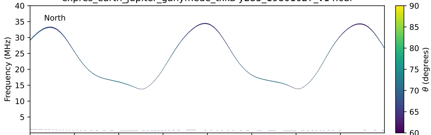
expres_earth_jupiter_ganymede_txka-y235_19801027_v14.cdf
