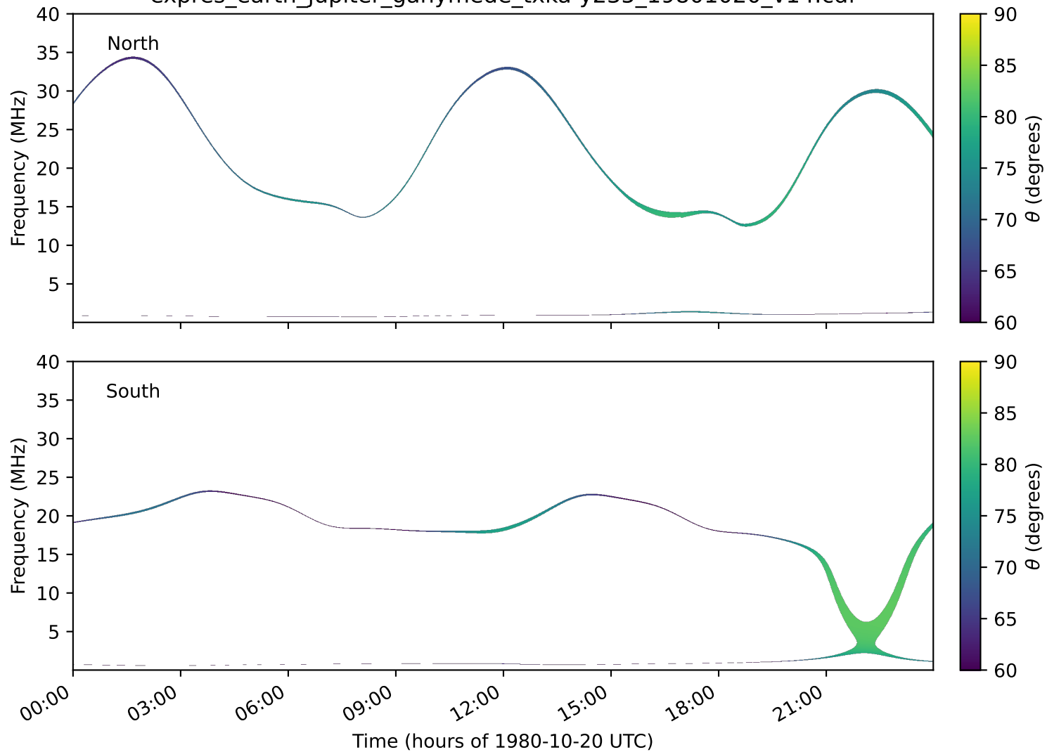
expres_earth_jupiter_ganymede_txka-y235_19801020_v14.cdf
