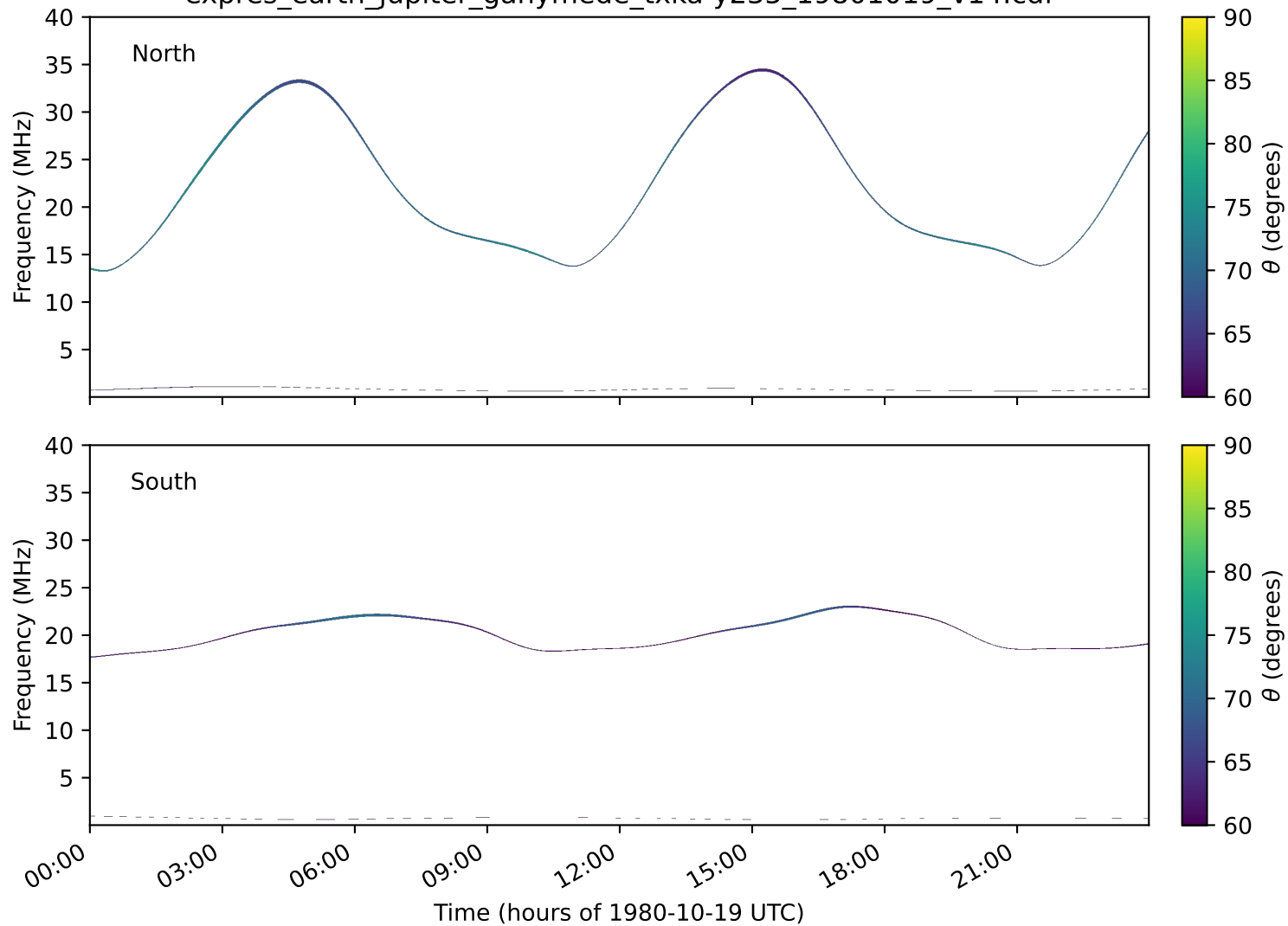
expres_earth_jupiter_ganymede_txka-y235_19801019_v14.cdf
