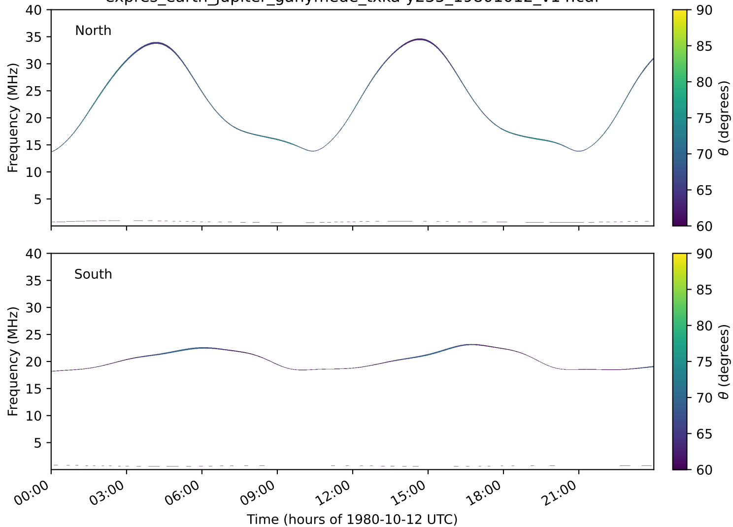
expres_earth_jupiter_ganymede_txka-y235_19801012_v14.cdf
