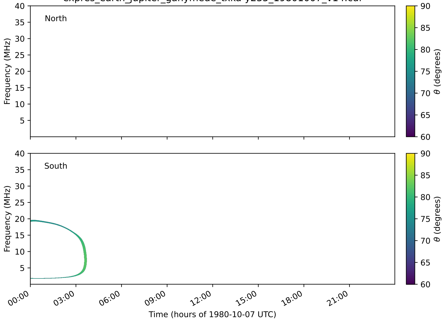
expres_earth_jupiter_ganymede_txka-y235_19801007_v14.cdf
