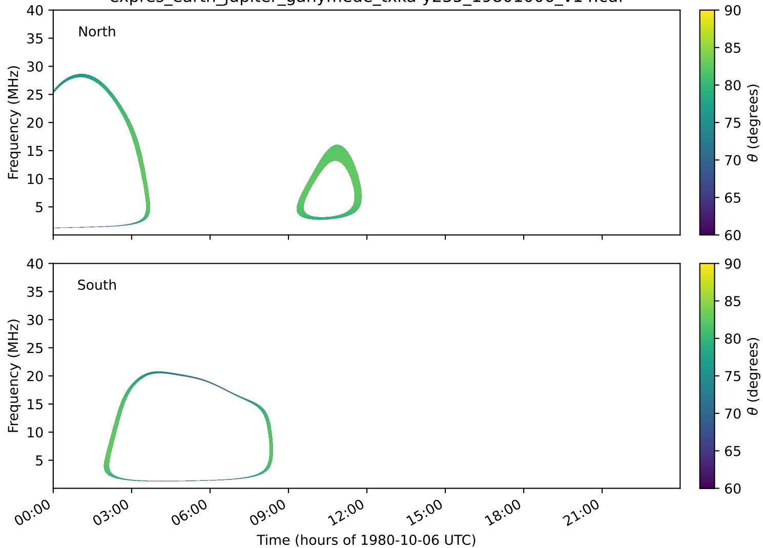
expres_earth_jupiter_ganymede_txka-y235_19801006_v14.cdf
