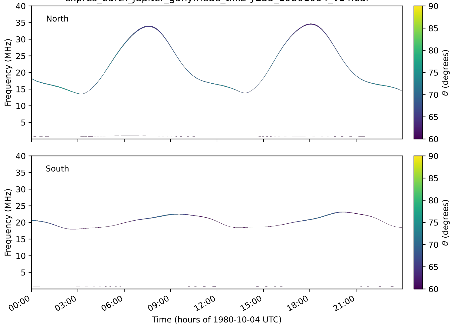
expres_earth_jupiter_ganymede_txka-y235_19801004_v14.cdf
