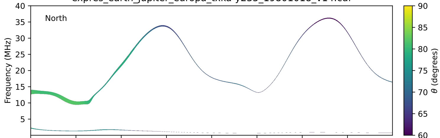
expres_earth_jupiter_europa_txka-y235_19801018_v14.cdf
