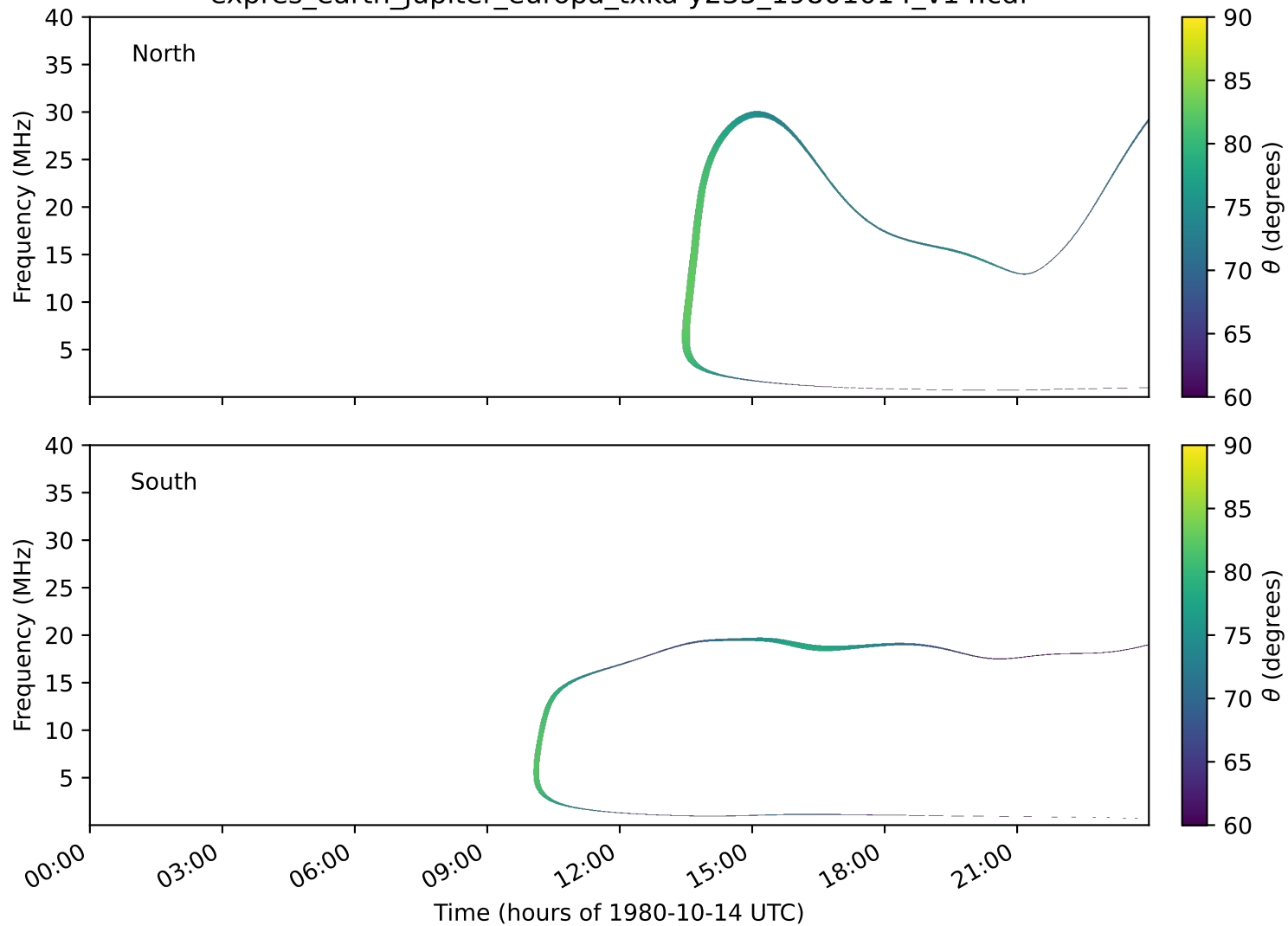
expres_earth_jupiter_europa_txka-y235_19801014_v14.cdf
