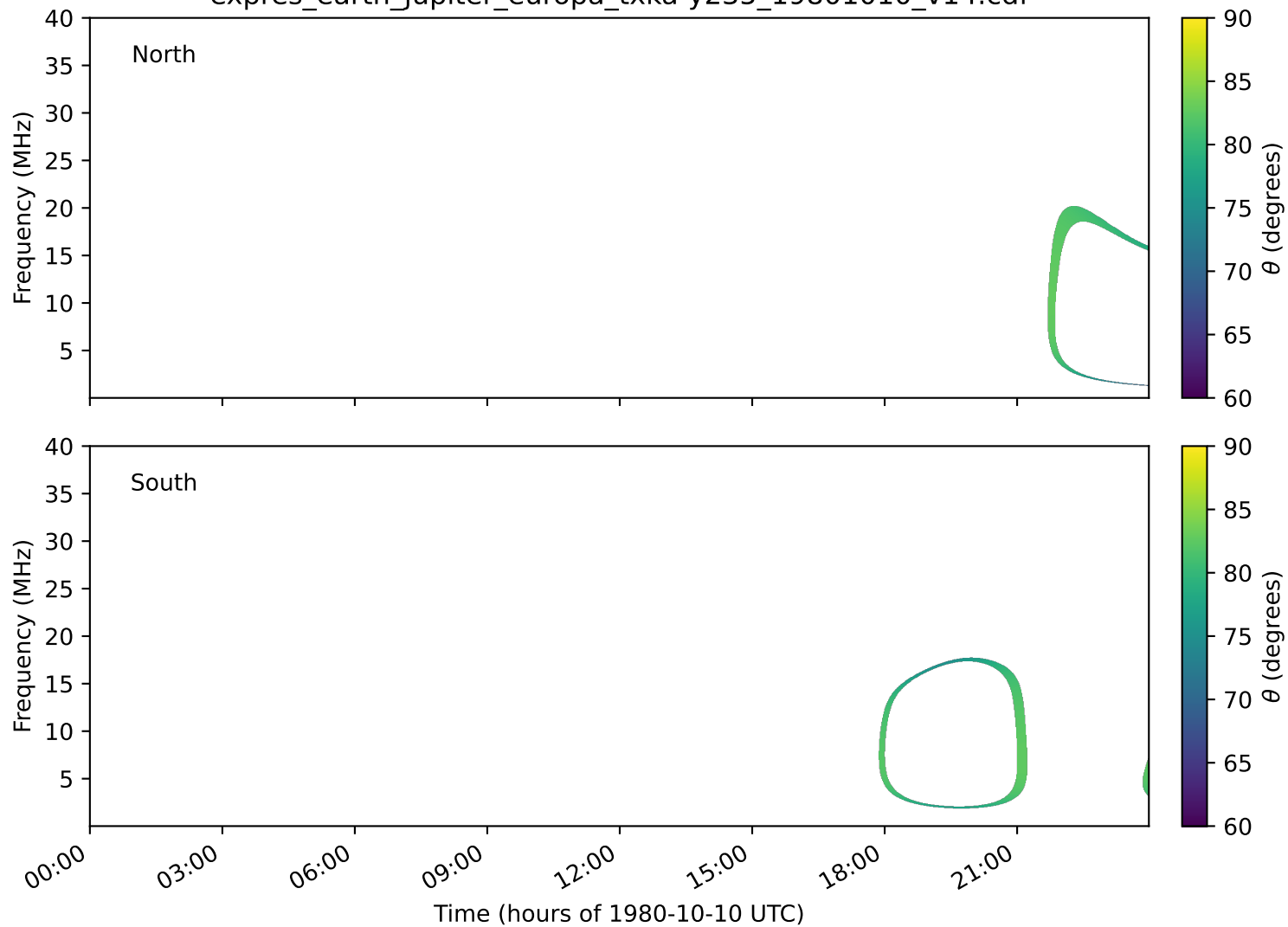
expres_earth_jupiter_europa_txka-y235_19801010_v14.cdf
