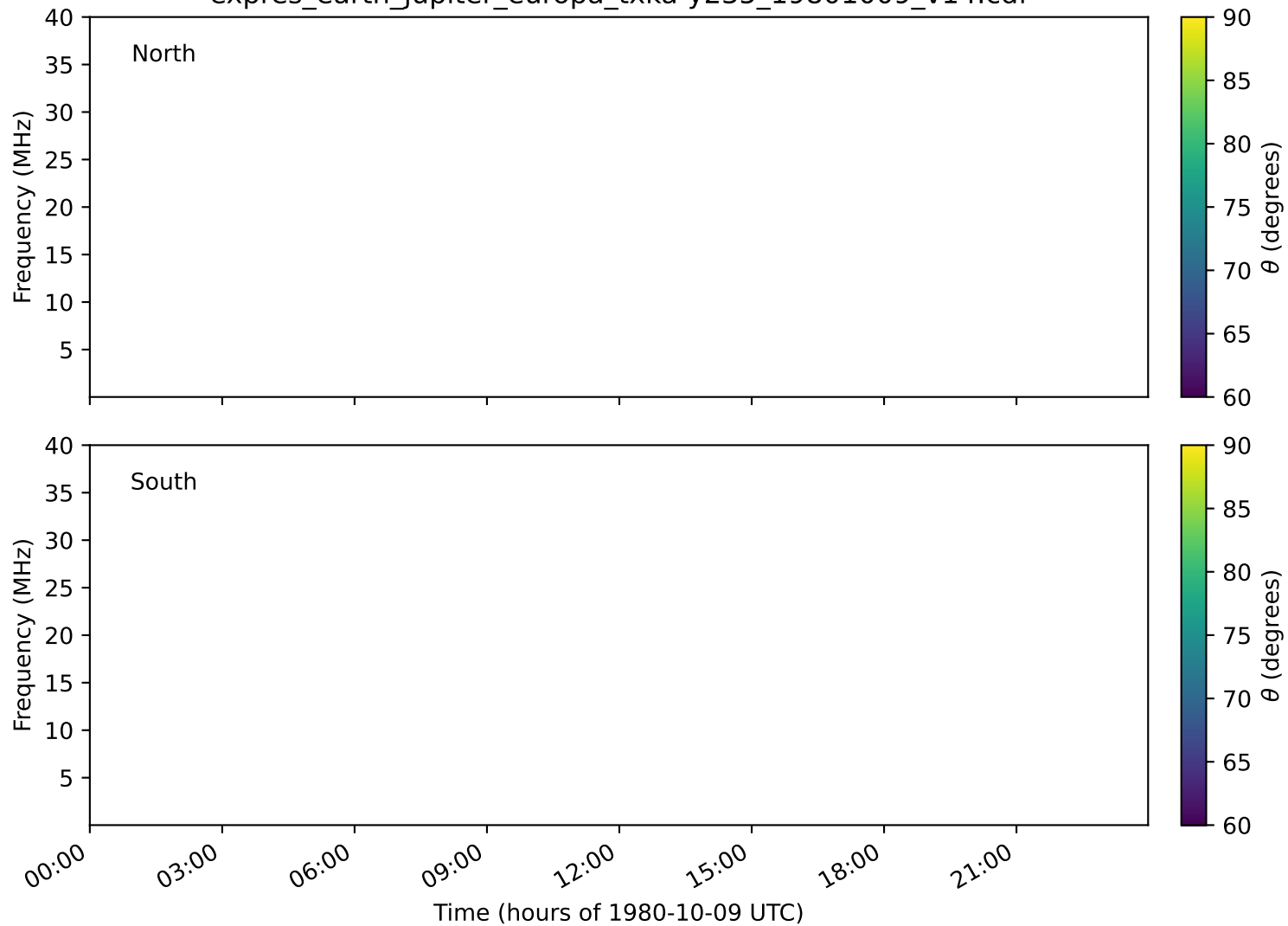
expres_earth_jupiter_europa_txka-y235_19801009_v14.cdf
