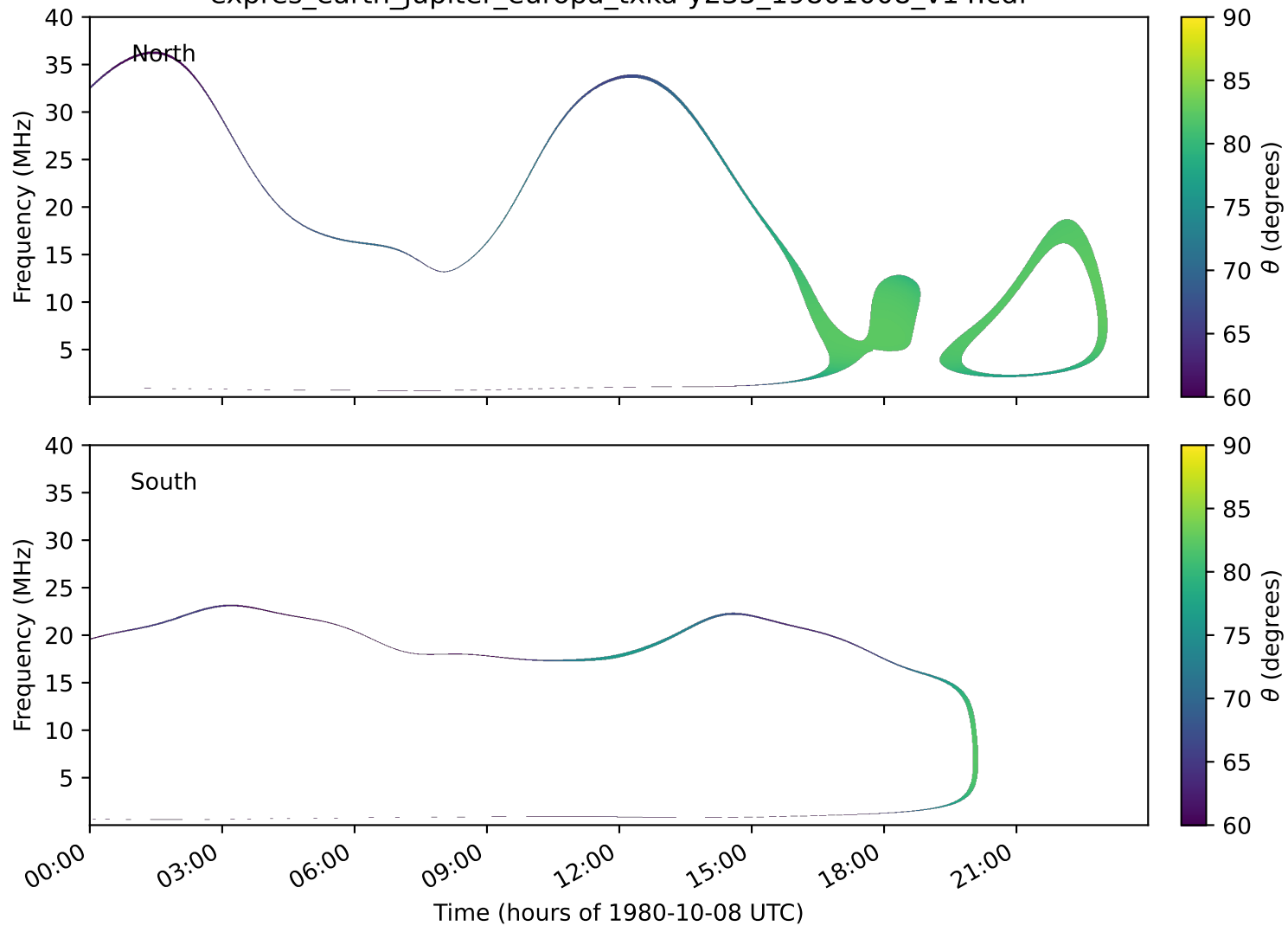
expres_earth_jupiter_europa_txka-y235_19801008_v14.cdf
