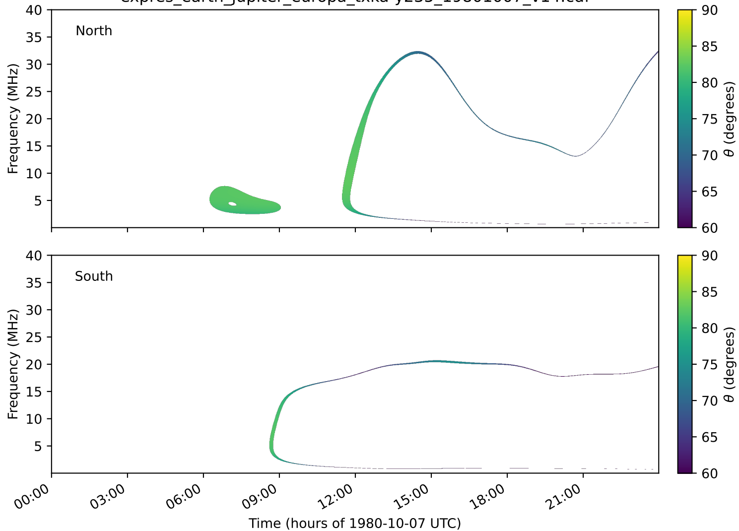
expres_earth_jupiter_europa_txka-y235_19801007_v14.cdf
