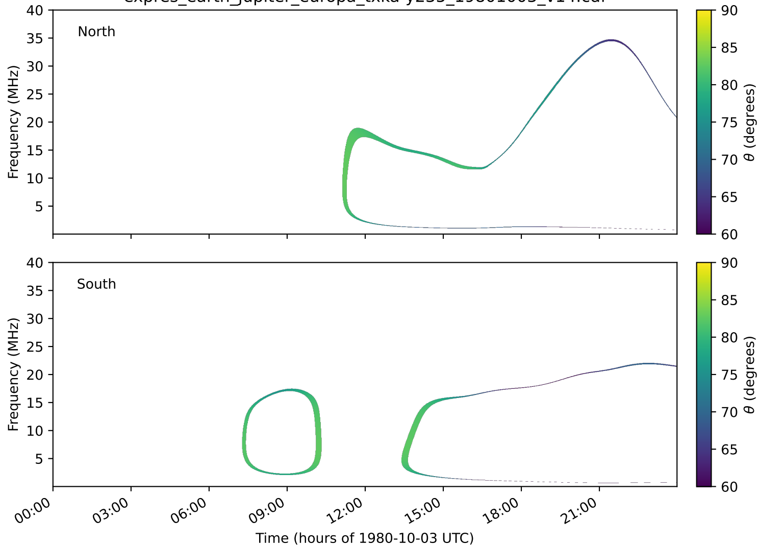
expres_earth_jupiter_europa_txka-y235_19801003_v14.cdf
