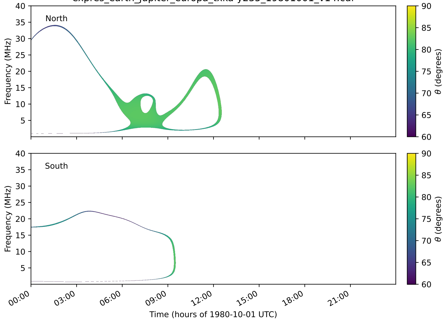
expres_earth_jupiter_europa_txka-y235_19801001_v14.cdf
