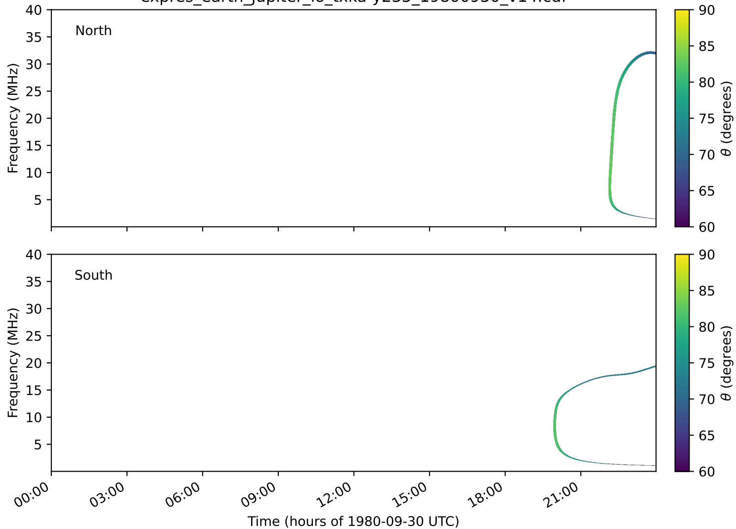
expres_earth_jupiter_io_txka-y235_19800930_v14.cdf
