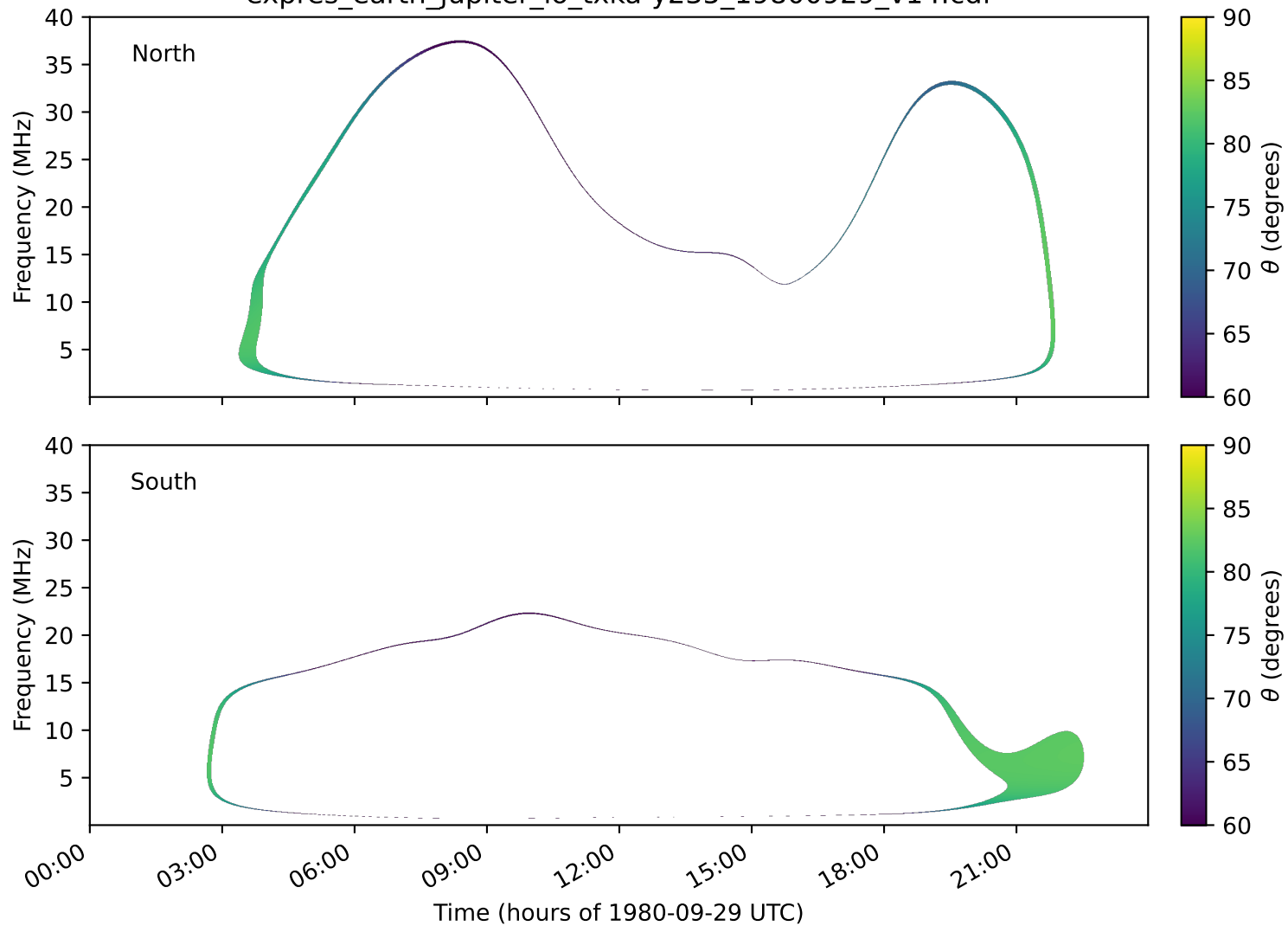
expres_earth_jupiter_io_txka-y235_19800929_v14.cdf
