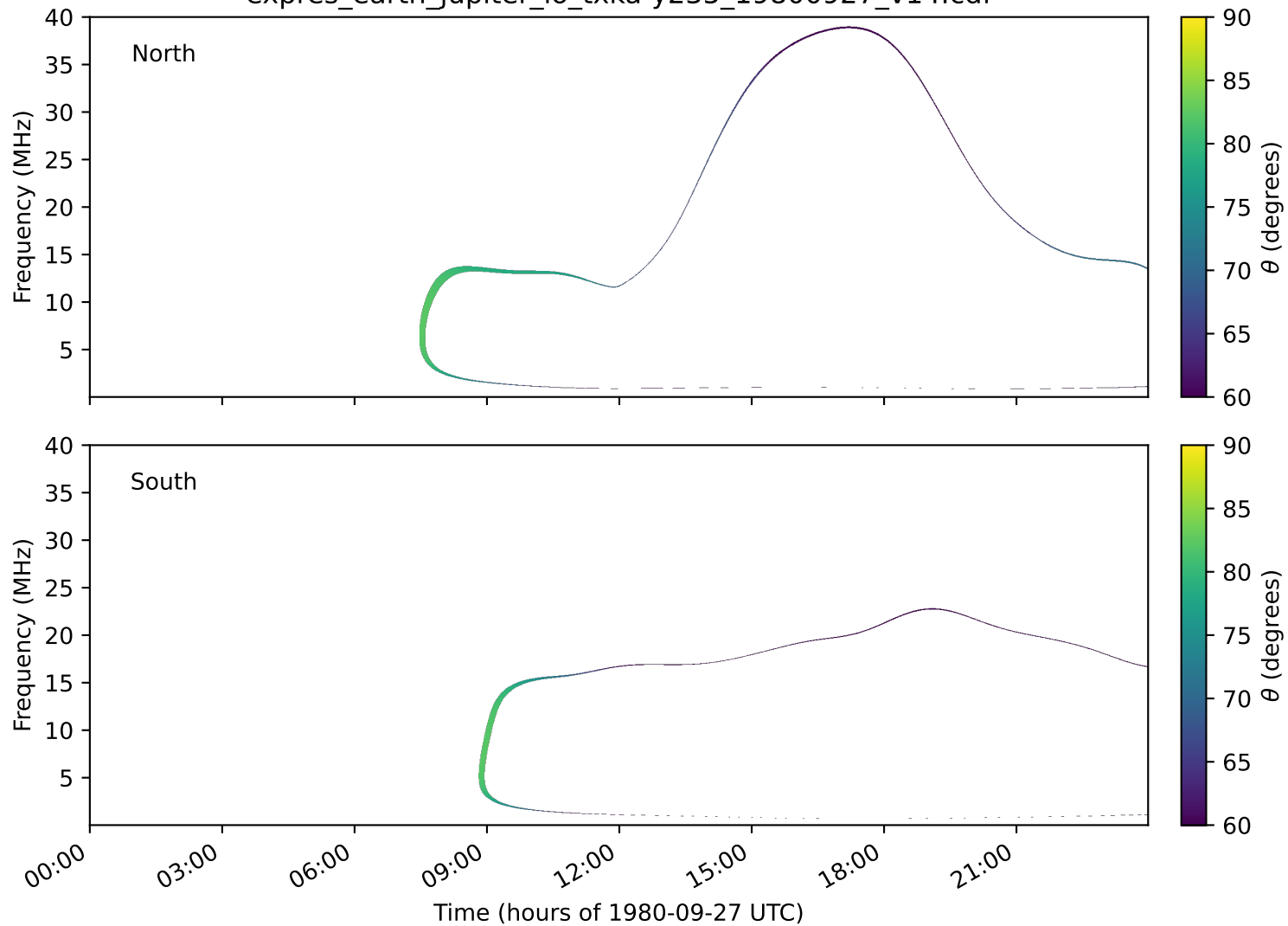
expres_earth_jupiter_io_txka-y235_19800927_v14.cdf
