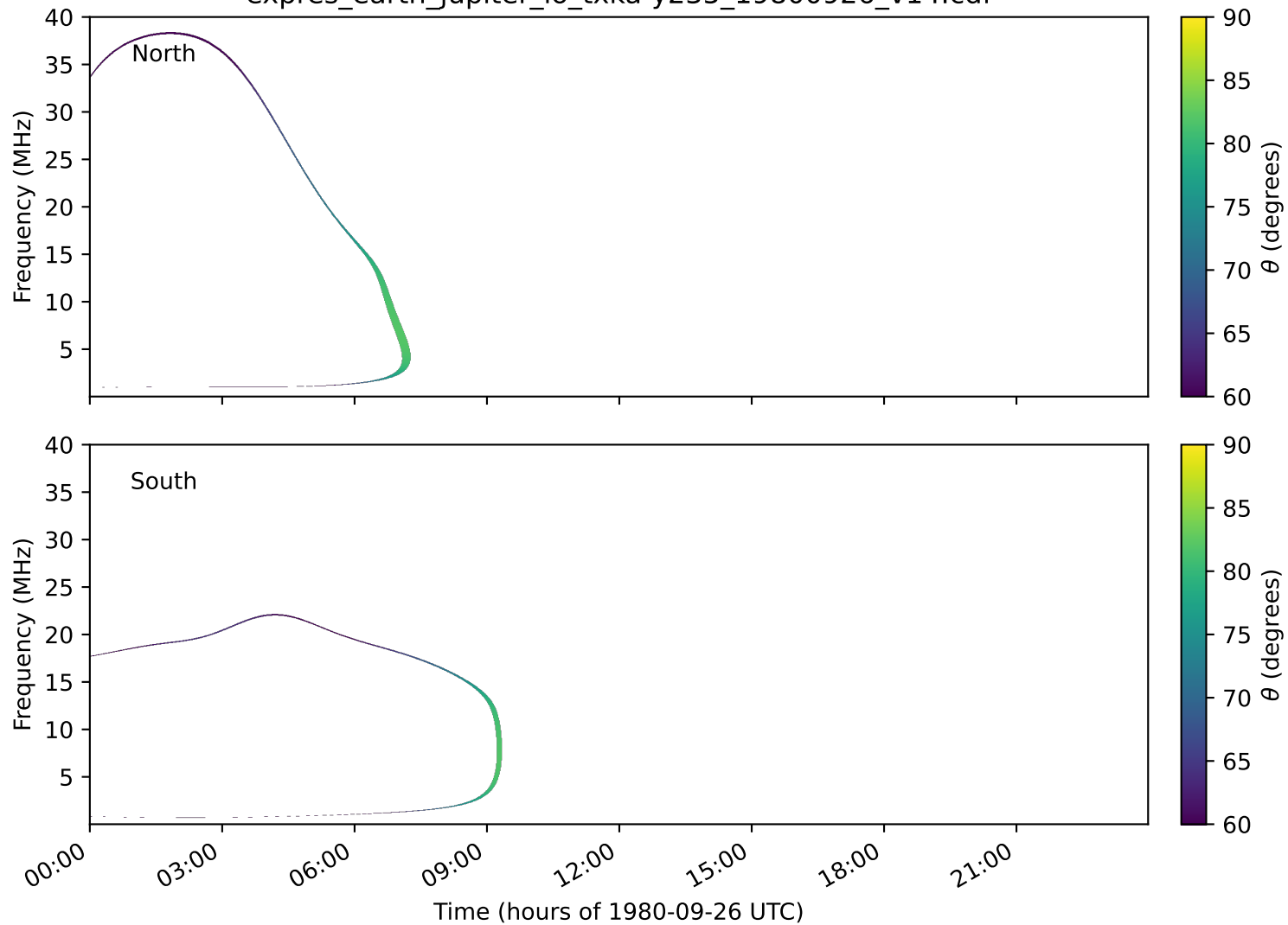
expres_earth_jupiter_io_txka-y235_19800926_v14.cdf
