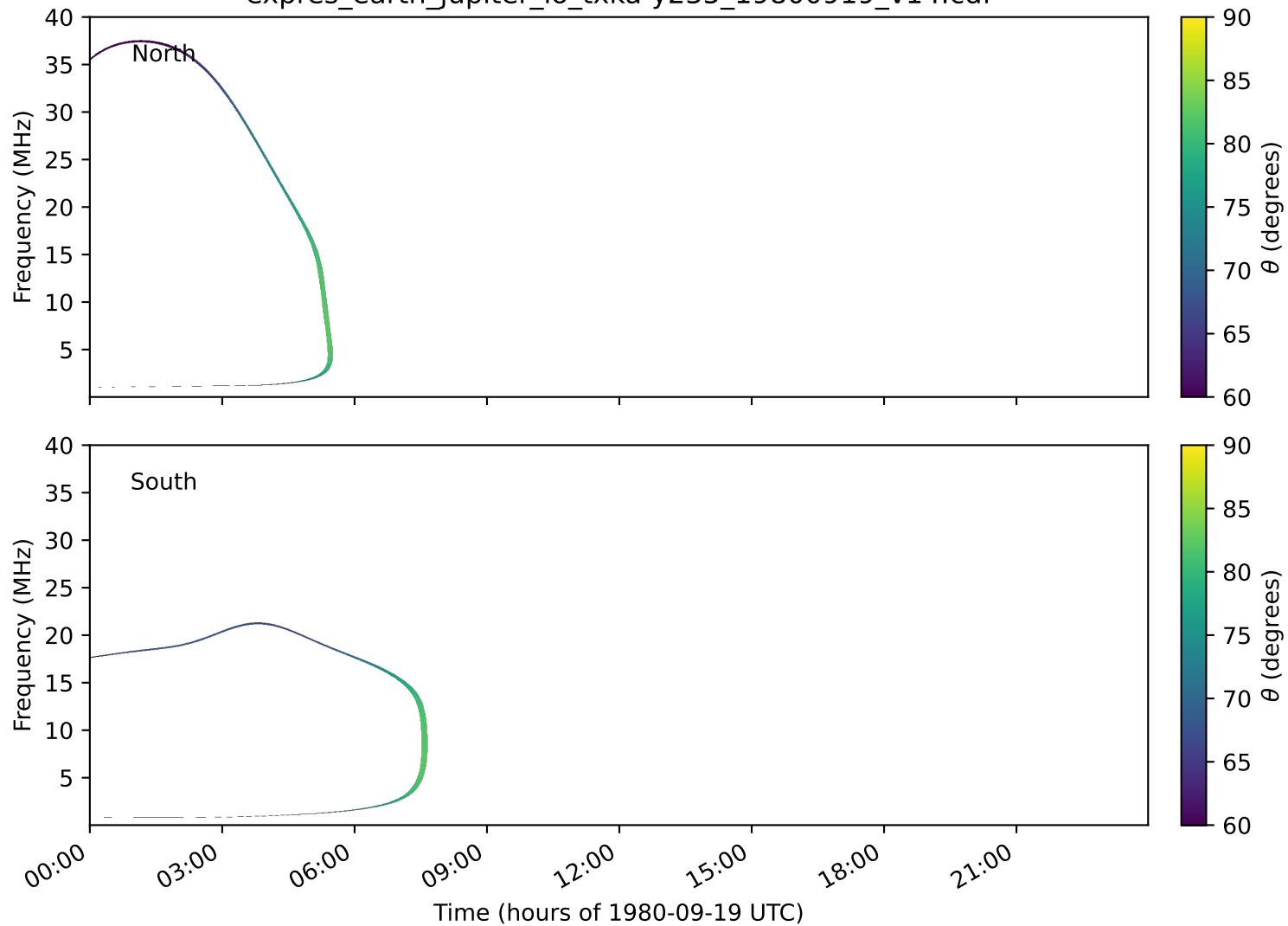
expres_earth_jupiter_io_txka-y235_19800919_v14.cdf
