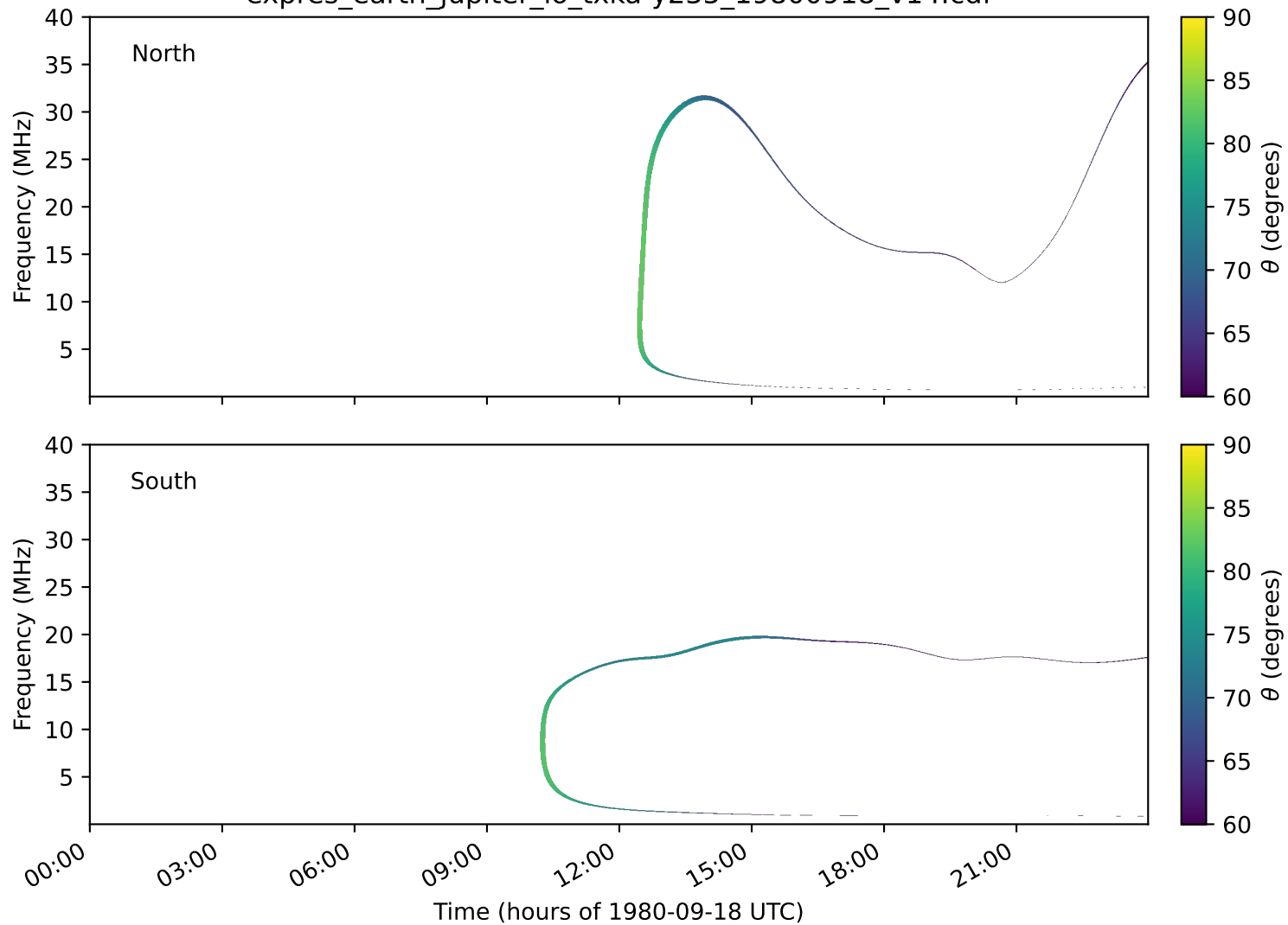
expres_earth_jupiter_io_txka-y235_19800918_v14.cdf
