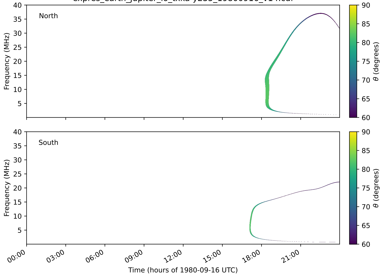
expres_earth_jupiter_io_txka-y235_19800916_v14.cdf
