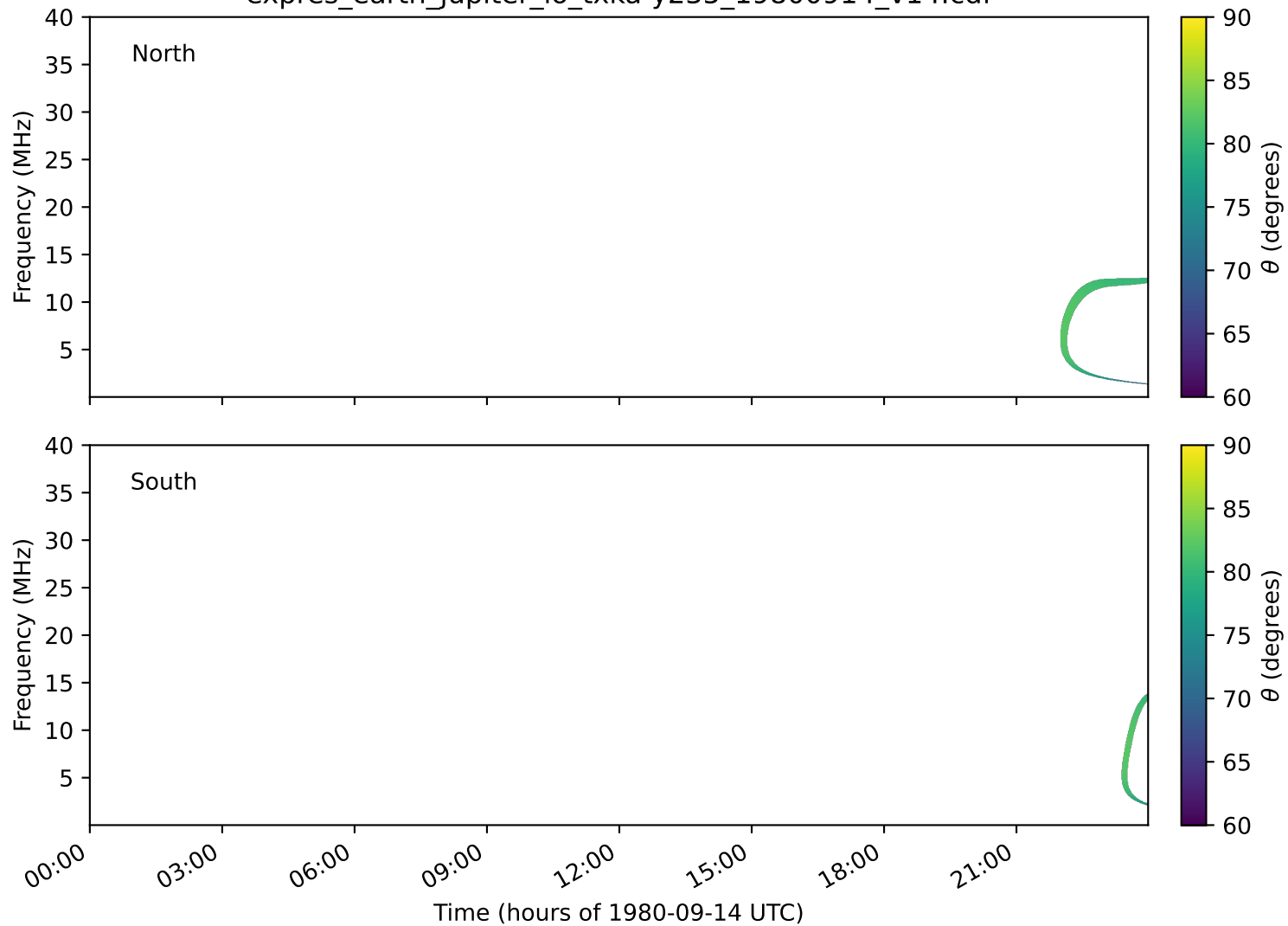
expres_earth_jupiter_io_txka-y235_19800914_v14.cdf
