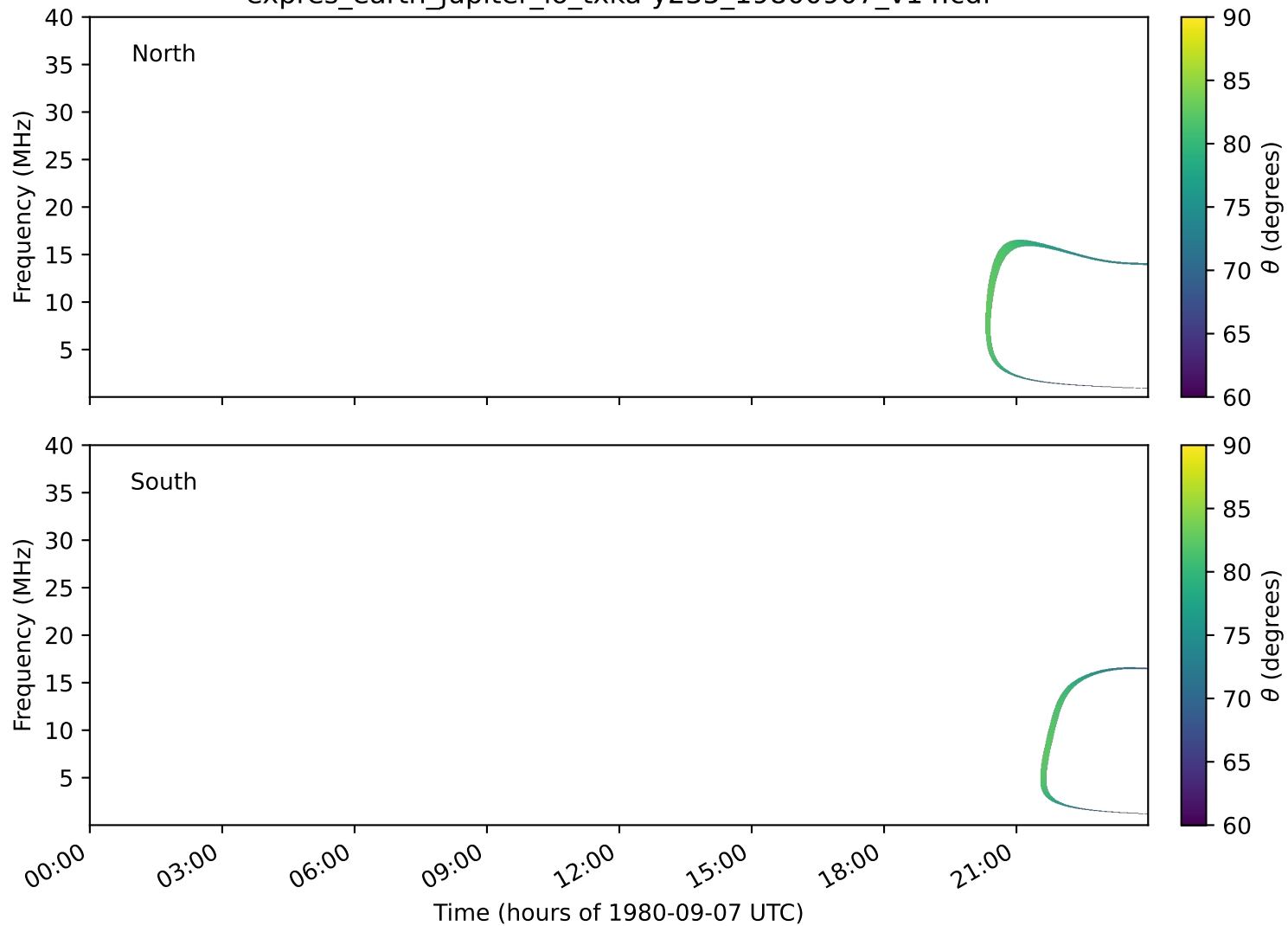
expres_earth_jupiter_io_txka-y235_19800907_v14.cdf
