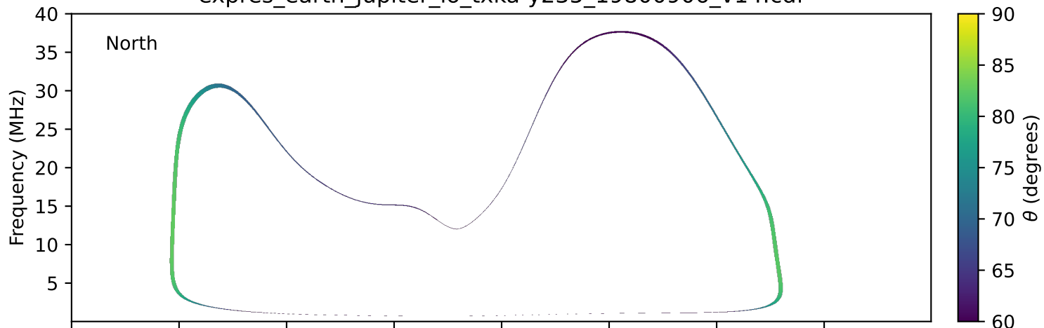
expres_earth_jupiter_io_txka-y235_19800906_v14.cdf
