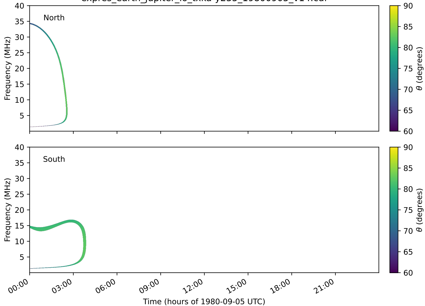
expres_earth_jupiter_io_txka-y235_19800905_v14.cdf
