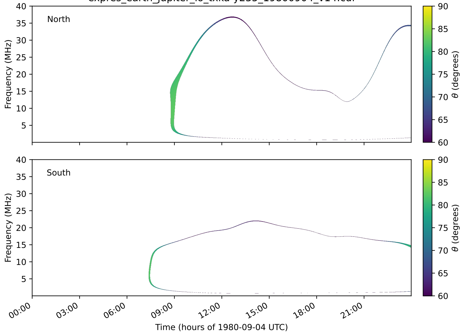
expres_earth_jupiter_io_txka-y235_19800904_v14.cdf
