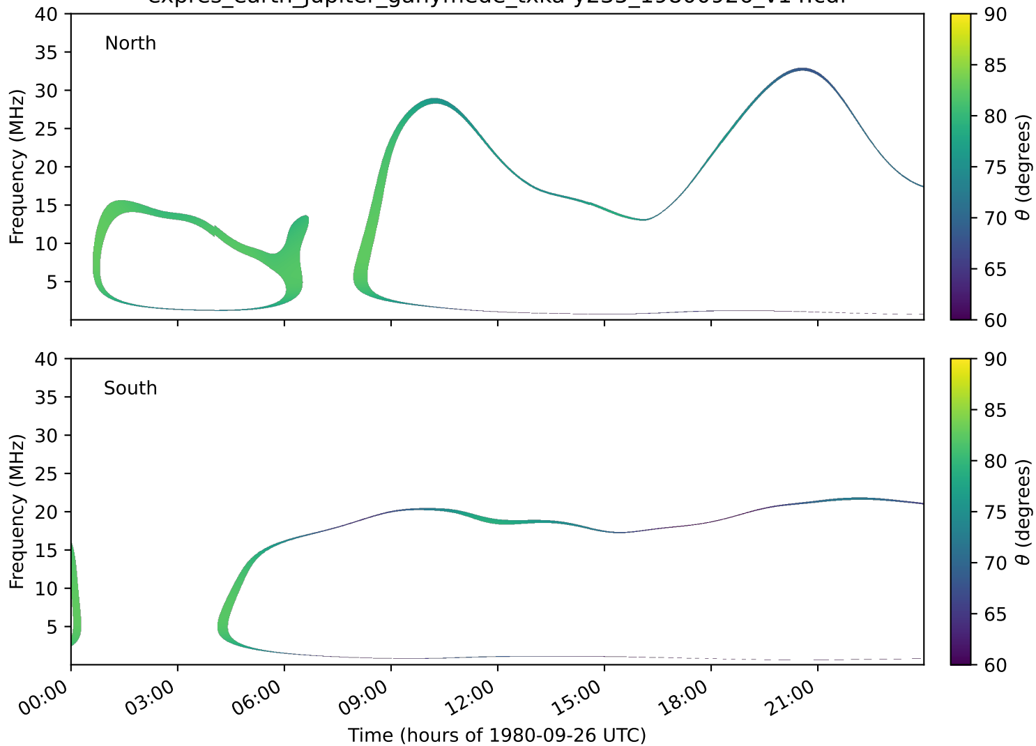
expres_earth_jupiter_ganymede_txka-y235_19800926_v14.cdf
