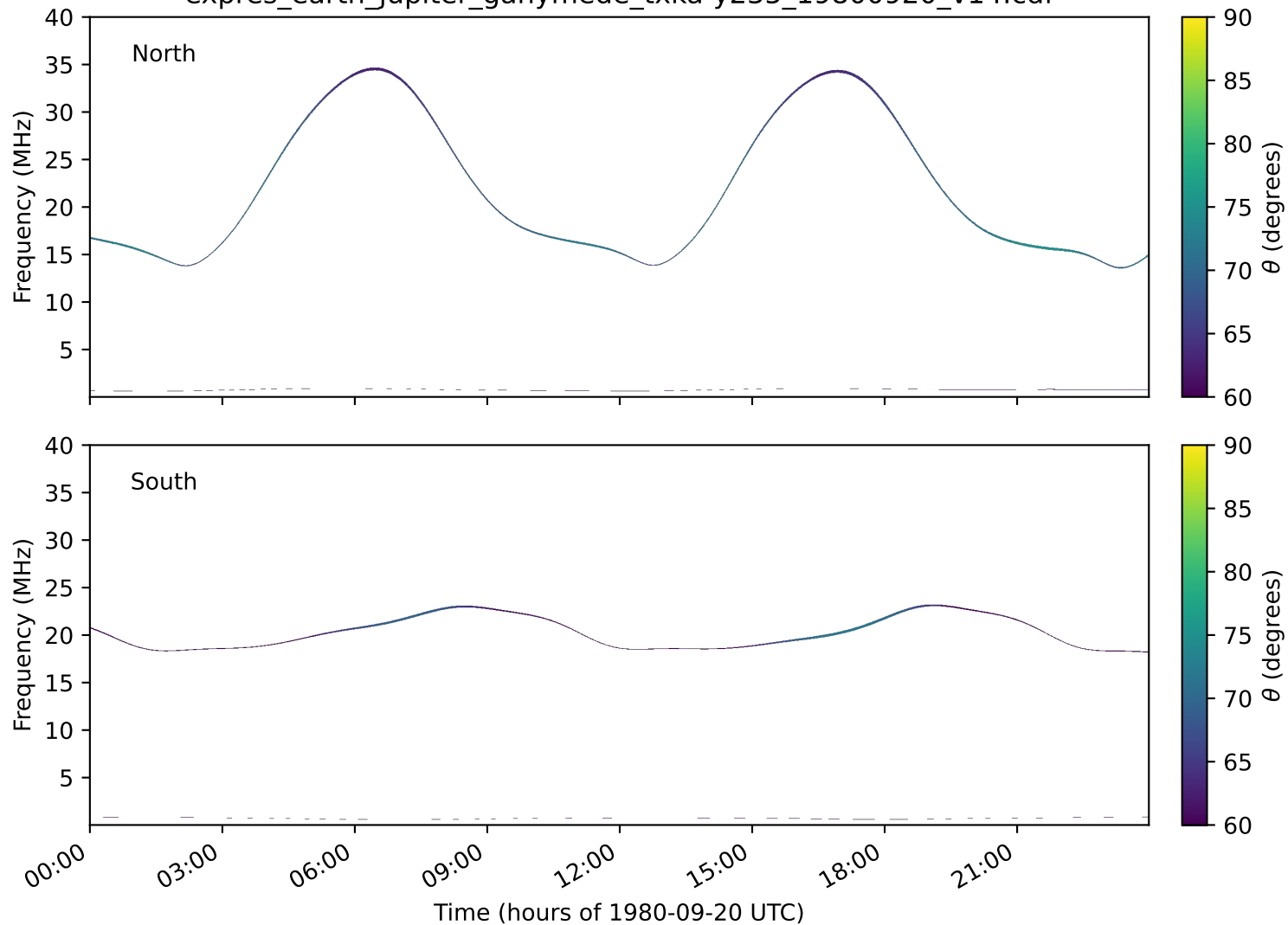
expres_earth_jupiter_ganymede_txka-y235_19800920_v14.cdf
