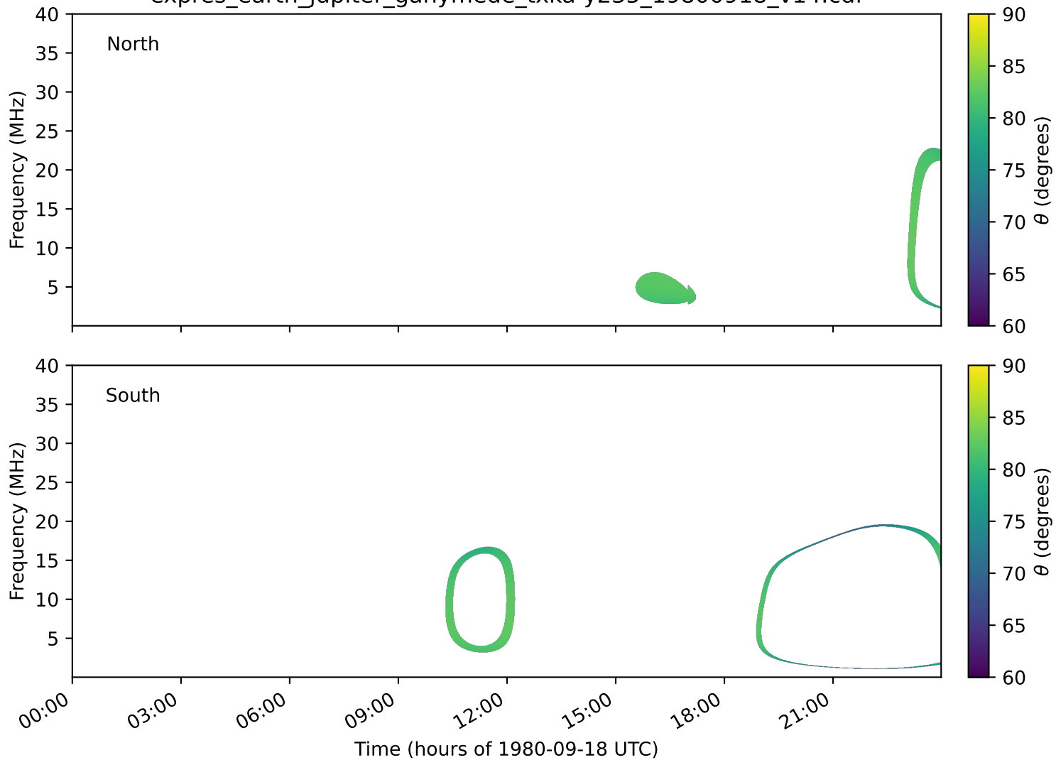
expres_earth_jupiter_ganymede_txka-y235_19800918_v14.cdf
