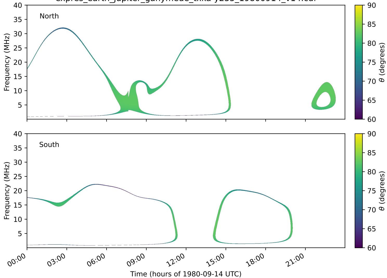
expres_earth_jupiter_ganymede_txka-y235_19800914_v14.cdf
