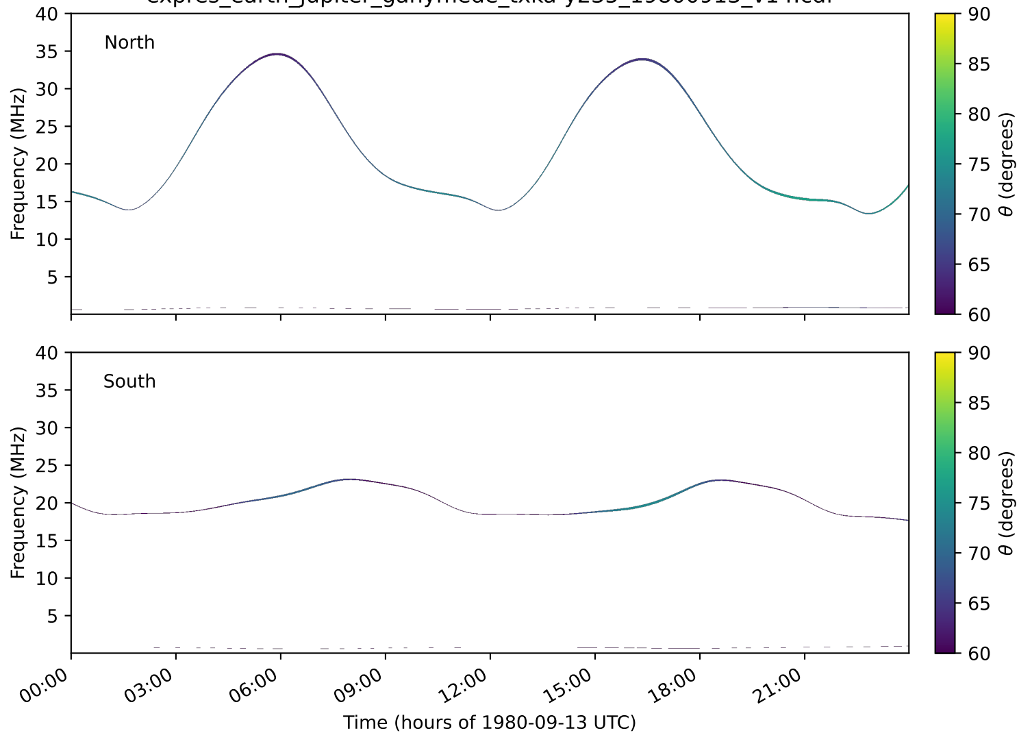
expres_earth_jupiter_ganymede_txka-y235_19800913_v14.cdf
