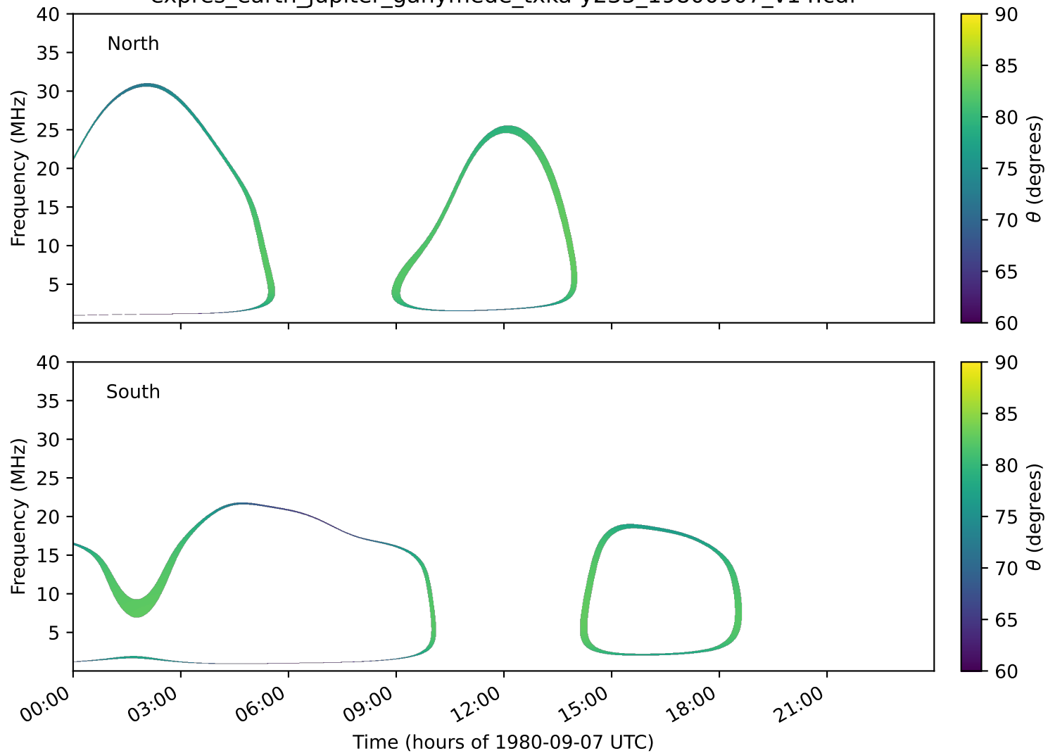
expres_earth_jupiter_ganymede_txka-y235_19800907_v14.cdf
