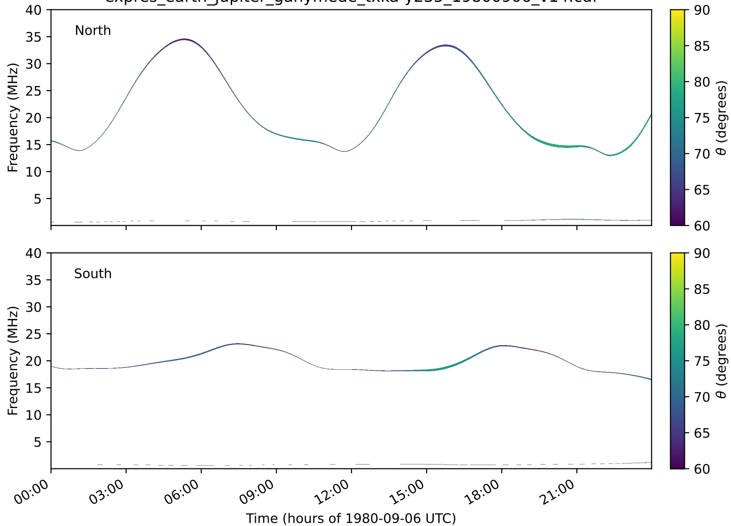
expres_earth_jupiter_ganymede_txka-y235_19800906_v14.cdf
