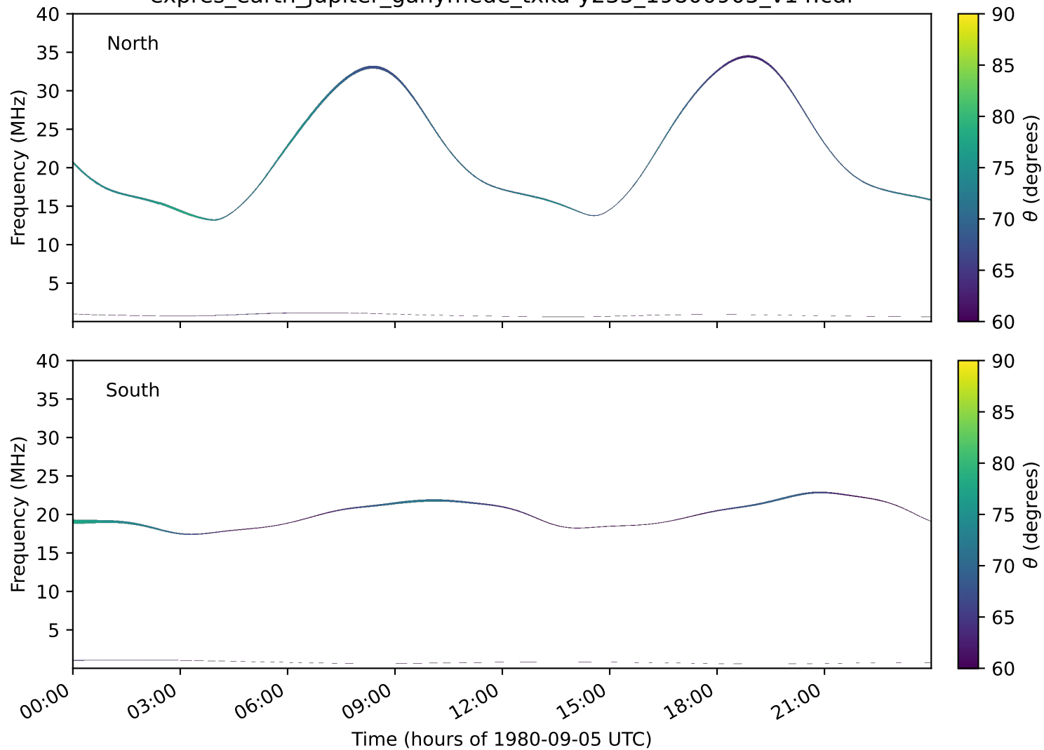
expres_earth_jupiter_ganymede_txka-y235_19800905_v14.cdf
