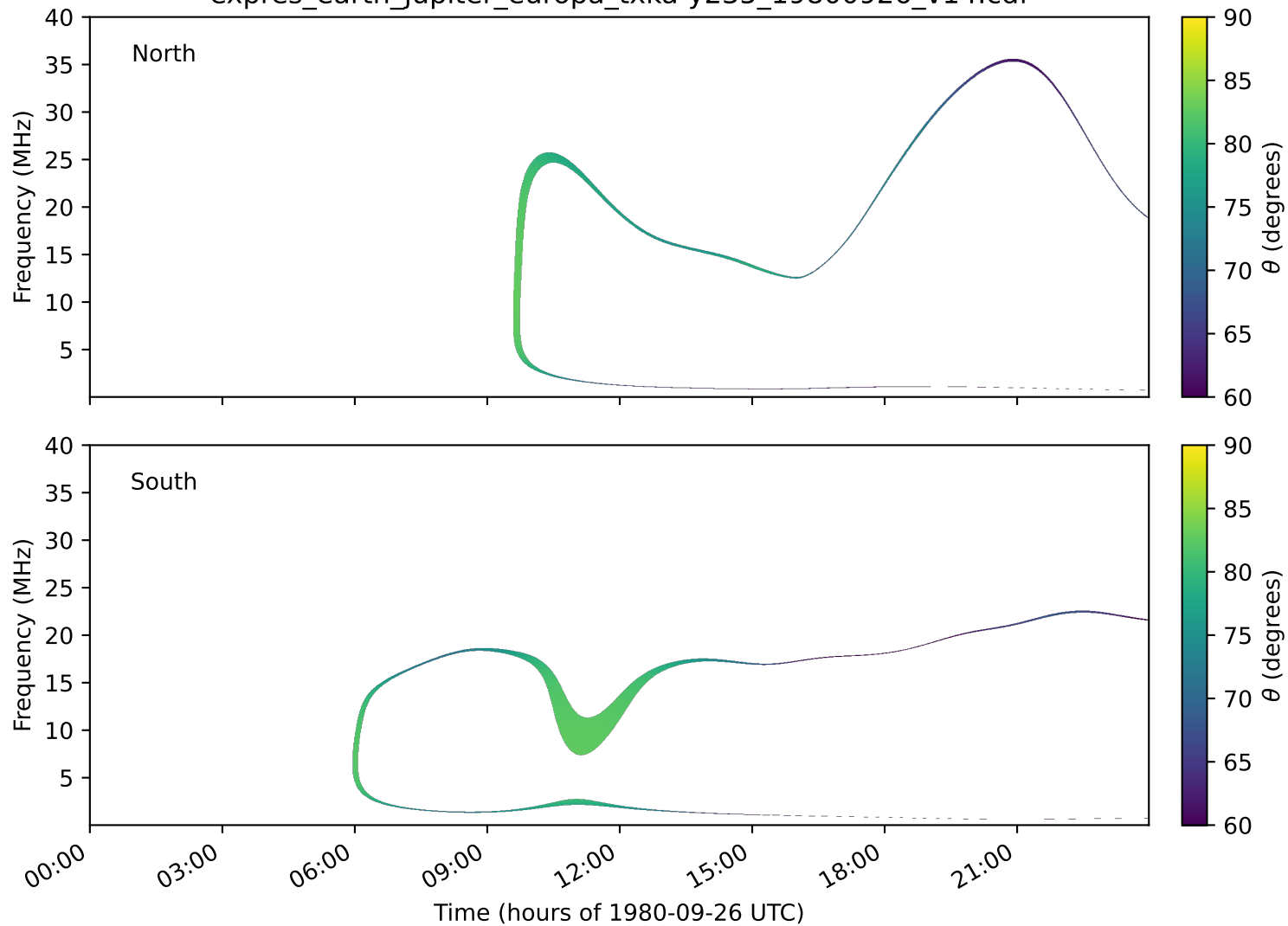
expres_earth_jupiter_europa_txka-y235_19800926_v14.cdf
