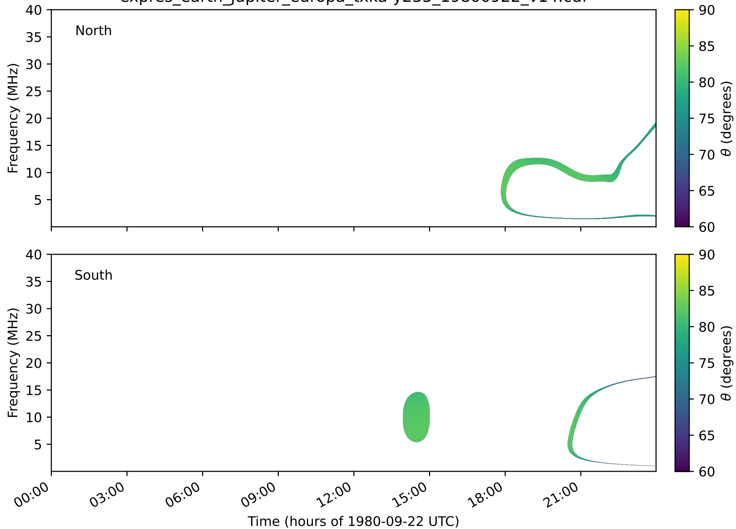
expres_earth_jupiter_europa_txka-y235_19800922_v14.cdf
