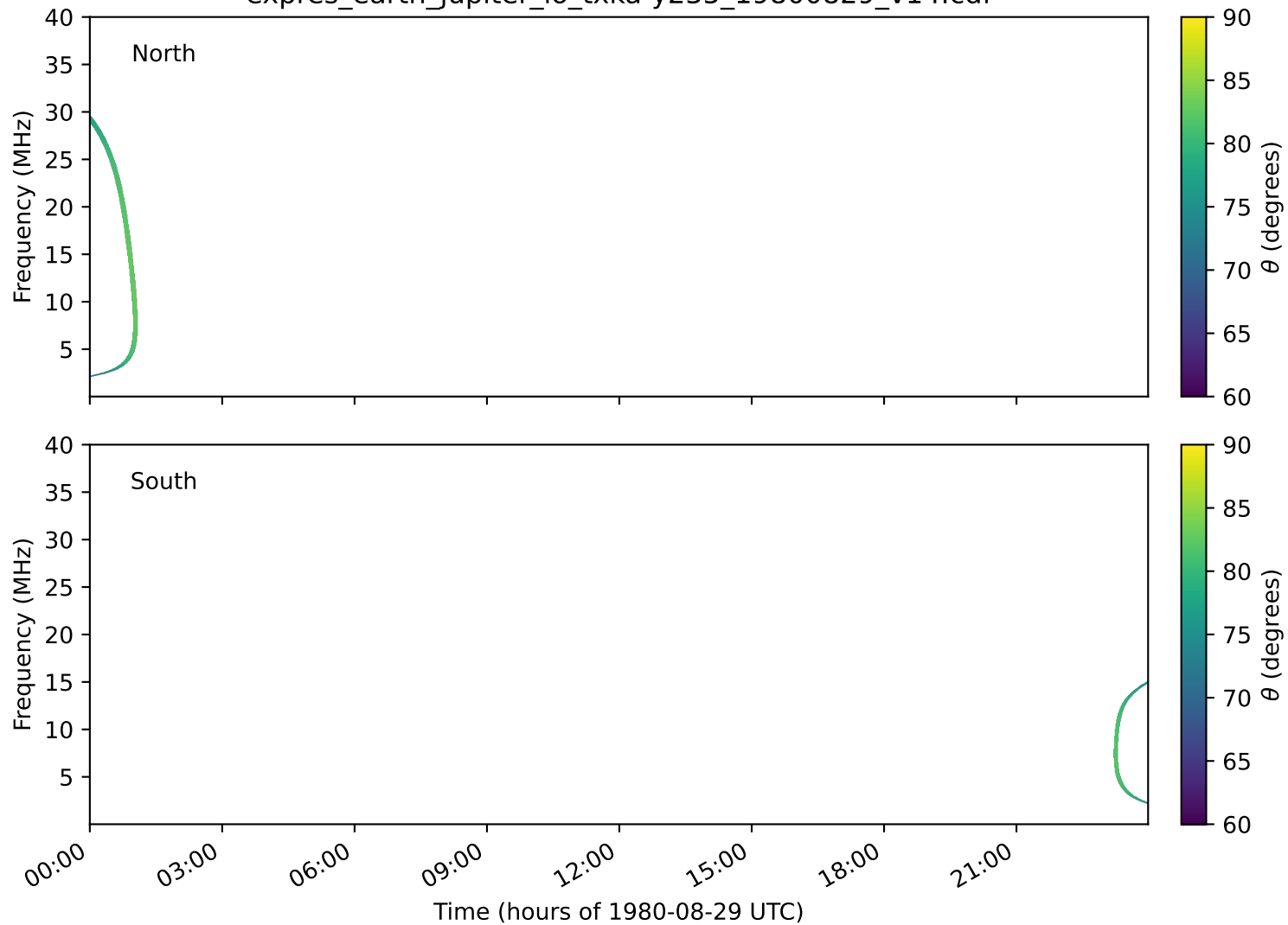
expres_earth_jupiter_io_txka-y235_19800829_v14.cdf
