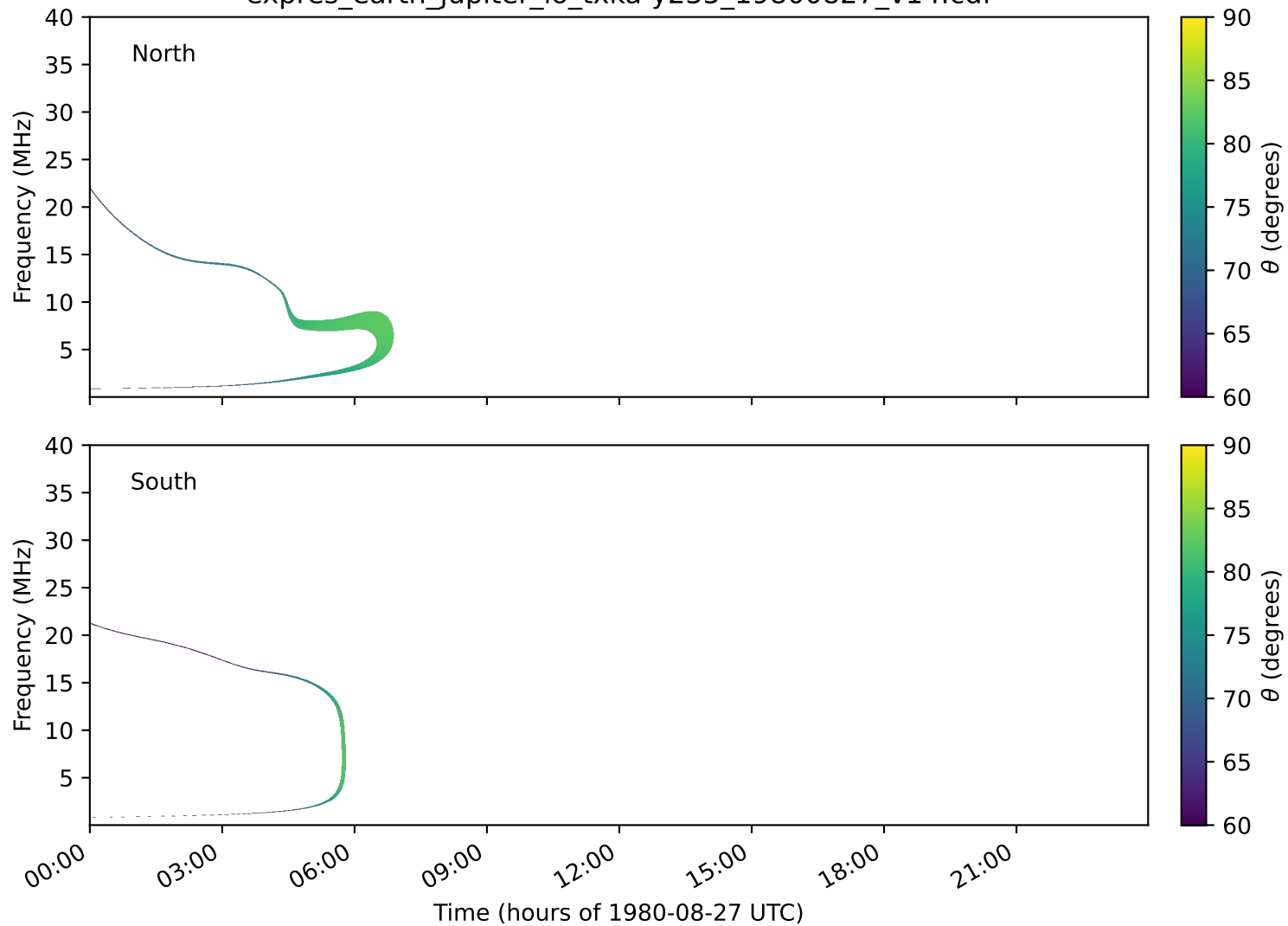
expres_earth_jupiter_io_txka-y235_19800827_v14.cdf
