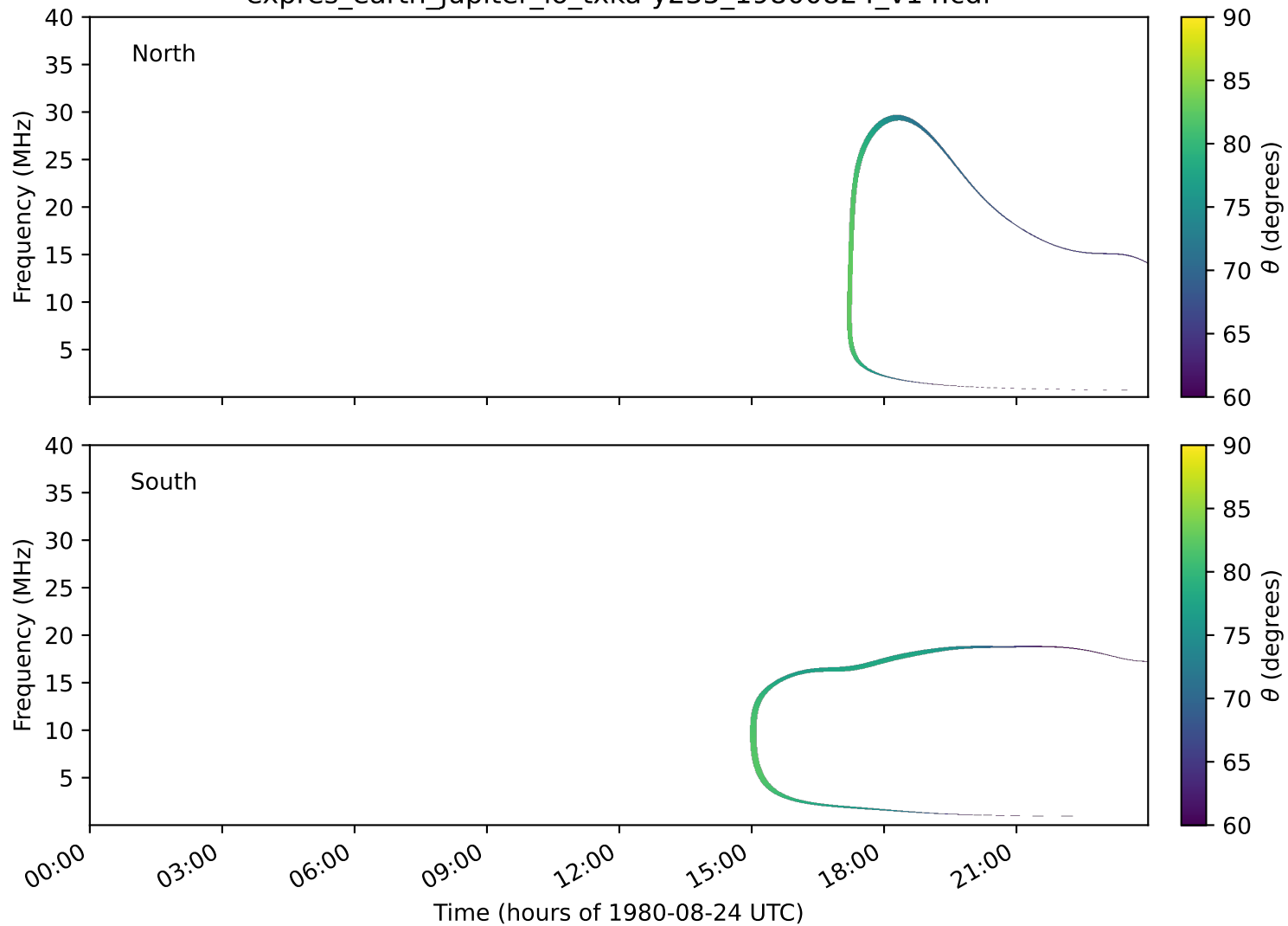
expres_earth_jupiter_io_txka-y235_19800824_v14.cdf
