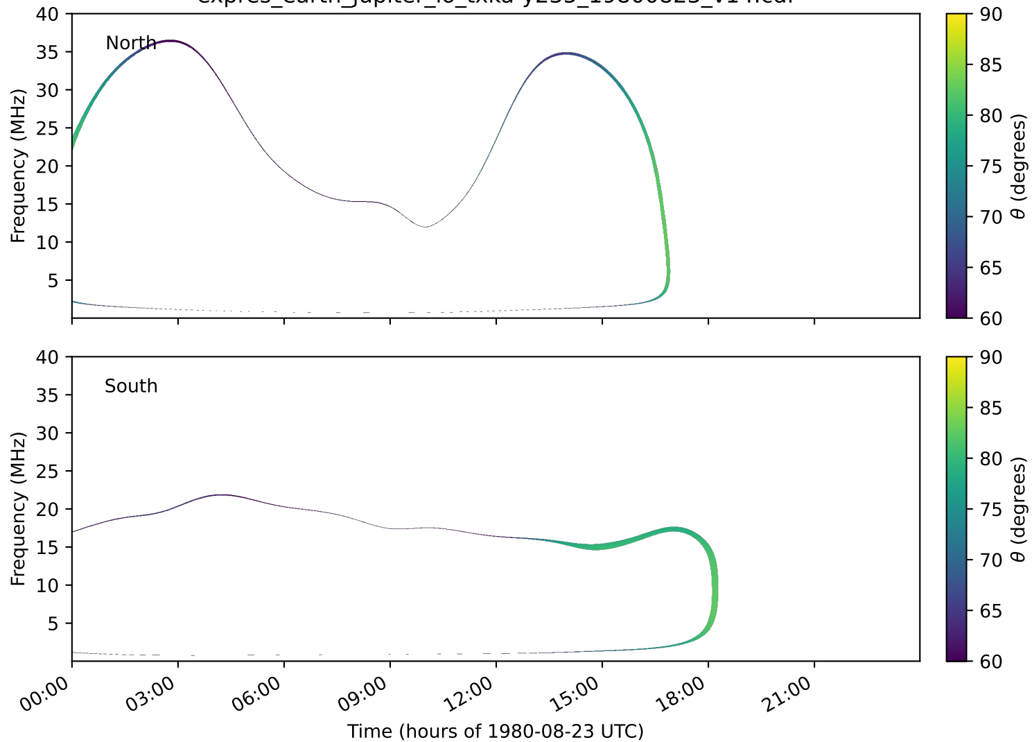
expres_earth_jupiter_io_txka-y235_19800823_v14.cdf
